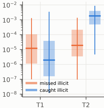
ensemble variance
