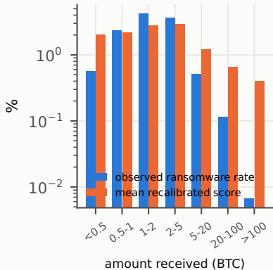
score vs. reality by amount
