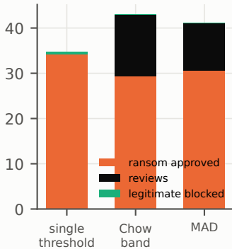
cost per 1,000 events (BTC)
