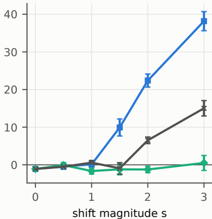
\pi_4 (MAD)
