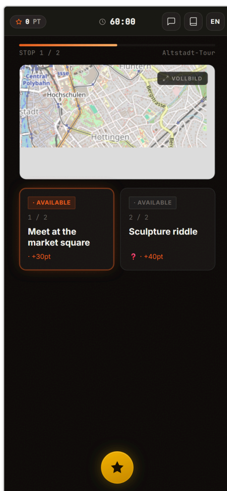
CityRush player home: mini-map, progress bar and mission tiles in route order.
