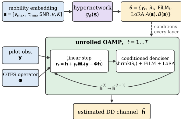
(b) Per-vehicle conditioned unfolding estimator
