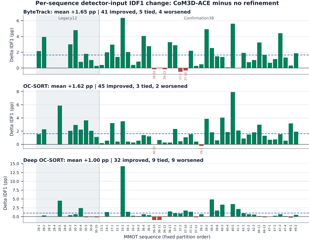
Figure 3: Per-sequence detector-input IDF1 change over all 50 MMOT test sequences. Each bar is CoM3D-ACE minus no refinement in percentage points, and the dashed line is the equal-sequence mean. Panels use the same fixed sequence order; gray shading marks legacy12. Positive, zero, and negative outcomes are all retained. Values come from the same frozen official-detector inputs as Table 2.
