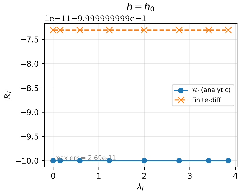
Exp 1 — Proposition 1: geometric functional \mathcal{R}_I
