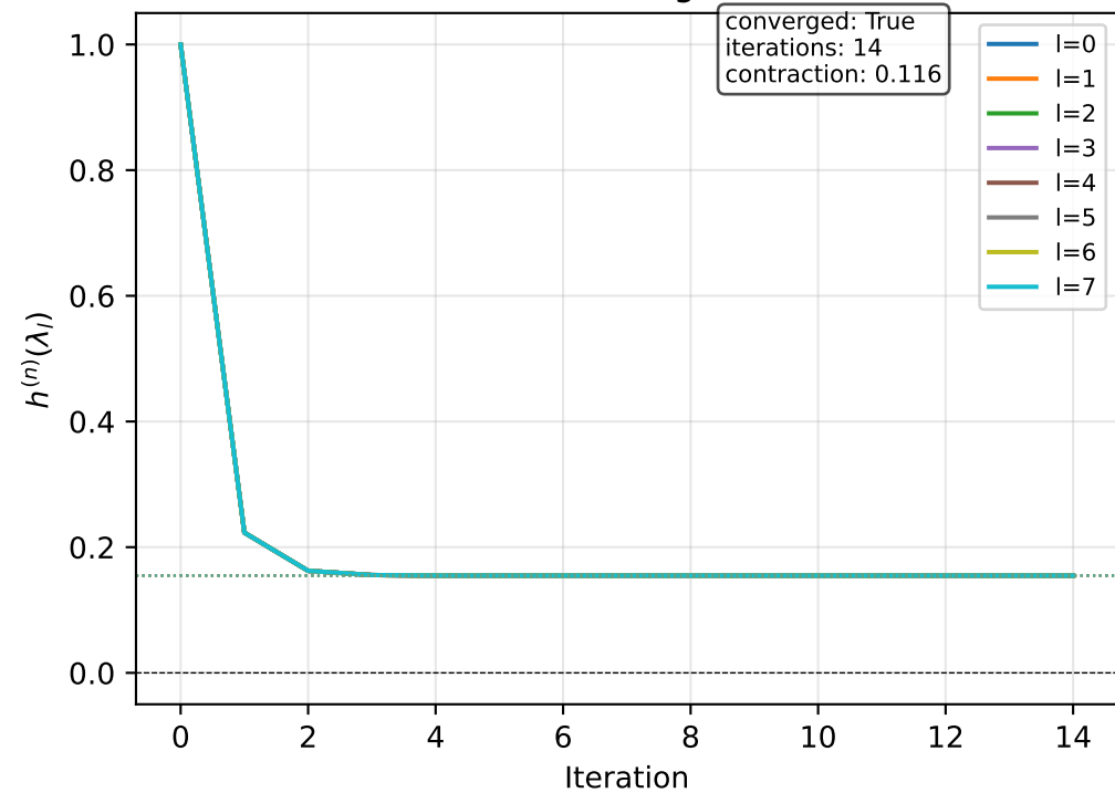
Per-mode convergence to h^*
