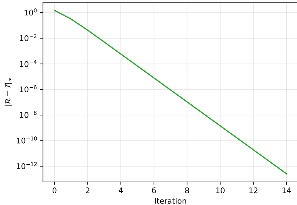
Field-equation residual
