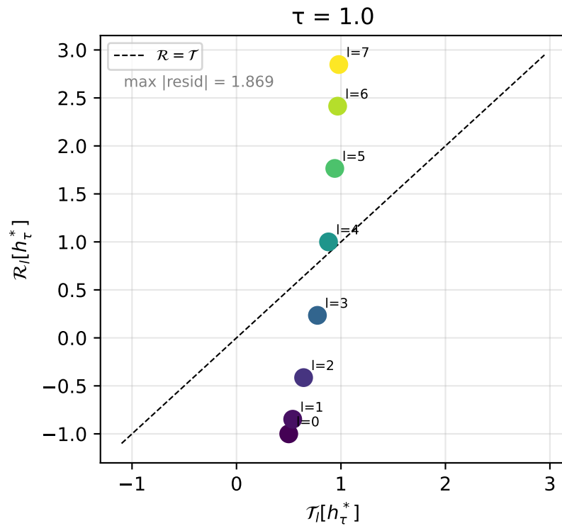
Exp 5 -- Remark 4: heat kernel \mathcal{R} vs \mathcal{T} (diagonal = exact fixed point)
