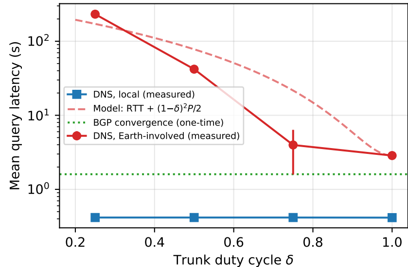
(a) Lunar ( P = 600 s)
