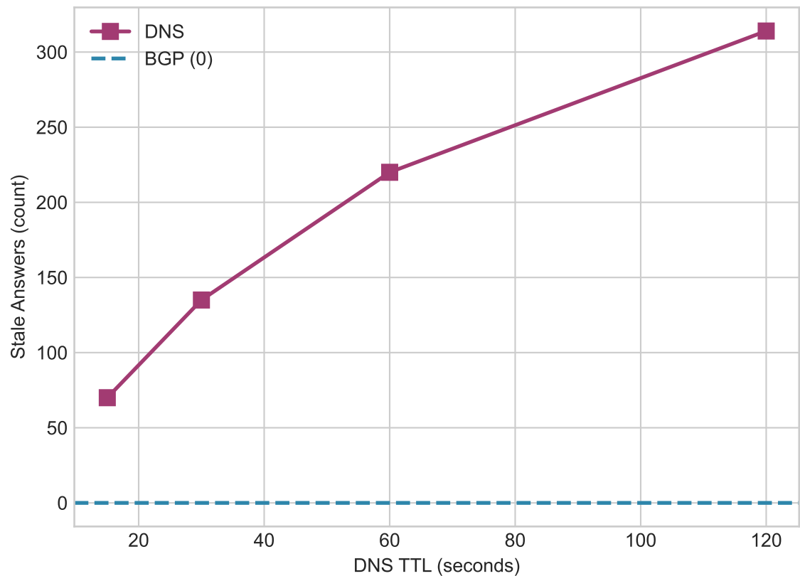
Stale Answers vs TTL
