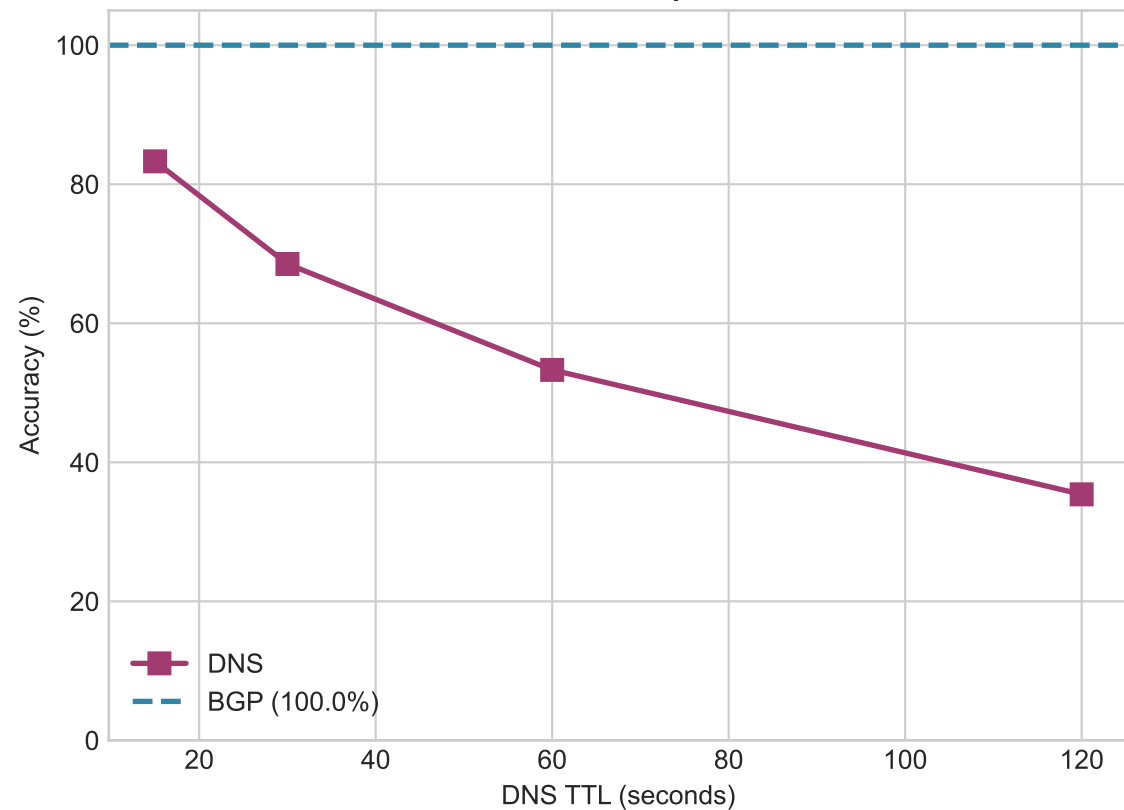
Answer Accuracy vs TTL
