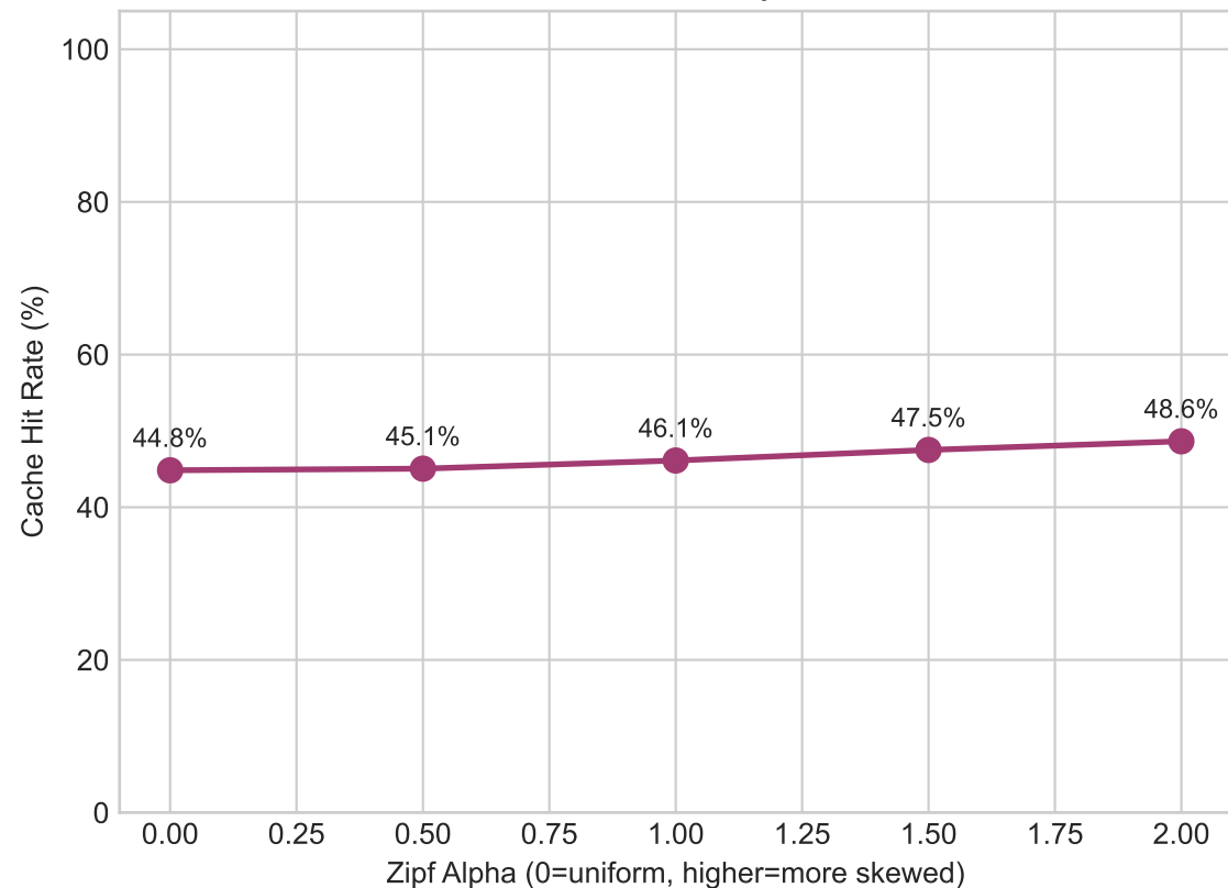
Cache Hit Rate vs Query Distribution
