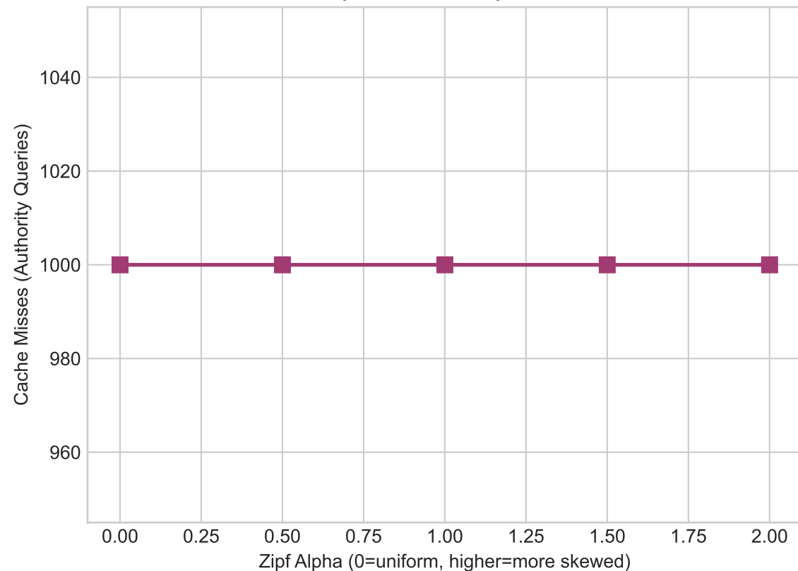
Authority Load vs Query Distribution
