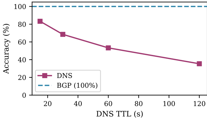
(a) Accuracy vs. TTL (churn=10 s)
