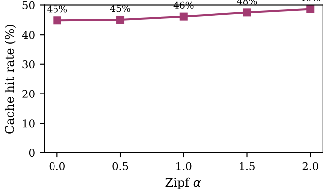
(b) Cache effectiveness
