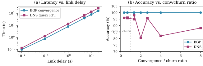
Fig. 5. Deep-space experiments. (a) Both BGP convergence and DNS query latency scale linearly with link delay; DNS pays 2 \times D \times d per query vs. BGP’s one-time D \times d . (b) DNS accuracy degrades when the convergence/churn ratio exceeds 1 (vertical line); BGP maintains 100%.
