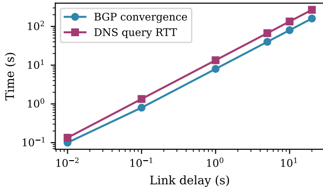
(a) Latency vs. link delay
