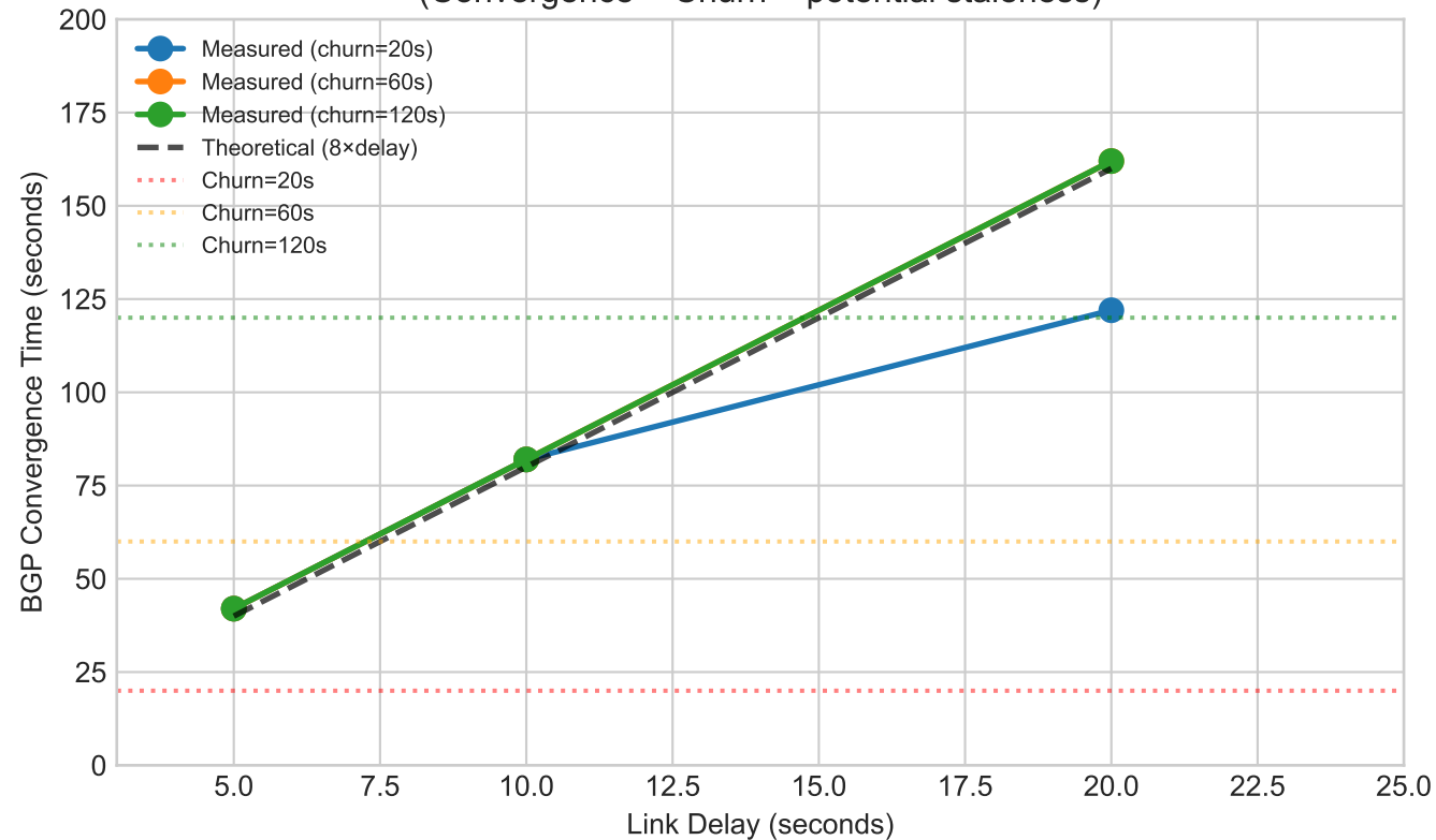
BGP Convergence Time vs Link Delay (Convergence > Churn = potential staleness)
