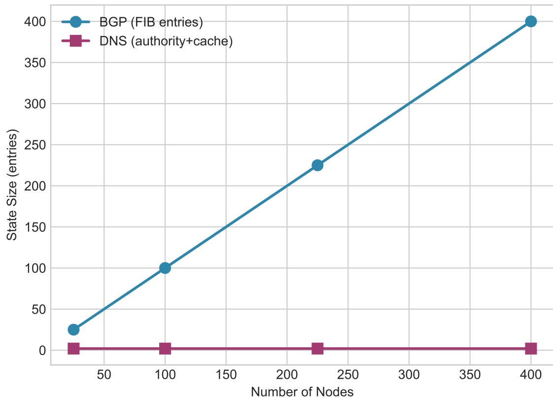
State Size vs Network Size
