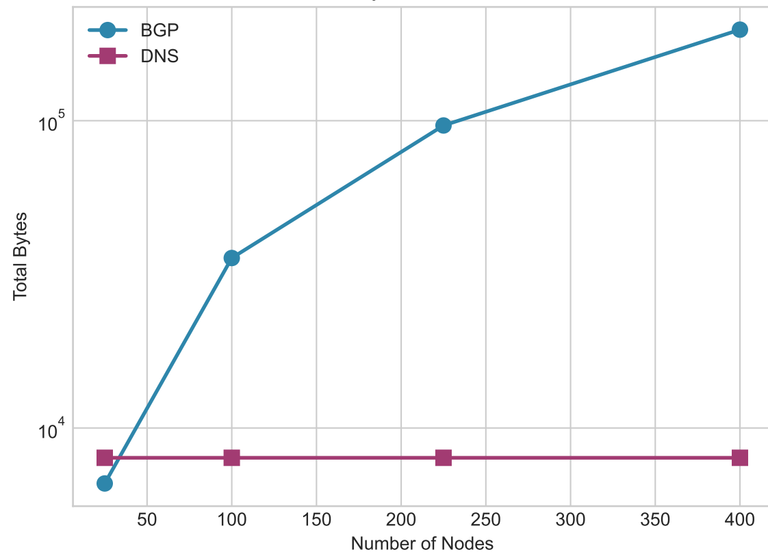
Network Bytes vs Network Size
