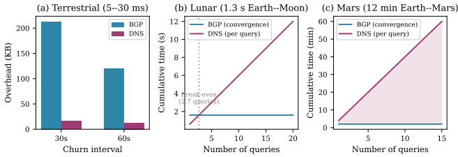
Fig. 7. Realistic deployment scenarios. (a) Terrestrial disaster response: DNS achieves 9–13× lower overhead. (b) Lunar network: BGP amortizes convergence after ~3 queries. (c) Mars network: DNS cumulative query time grows linearly while BGP remains flat after convergence.
