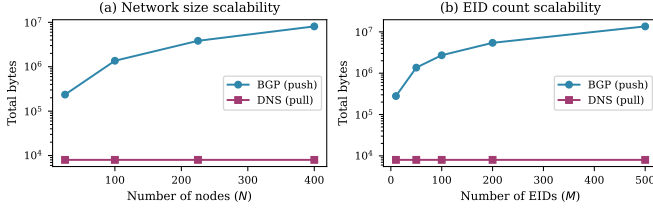
Fig. 2. Scalability of network overhead. (a) BGP overhead grows super-linearly with node count ( O(N^2) in a grid), while DNS remains constant. (b) BGP overhead scales linearly with EID count ( O(N \cdot M) ), while DNS overhead depends only on the query count.
