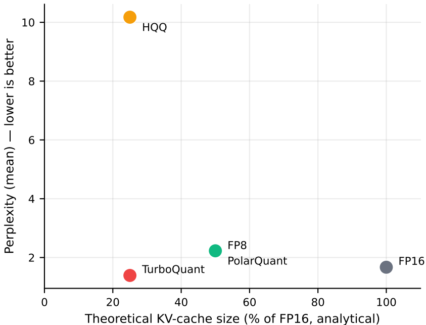
Quality vs theoretical KV-cache size @ 16,000 ctx
