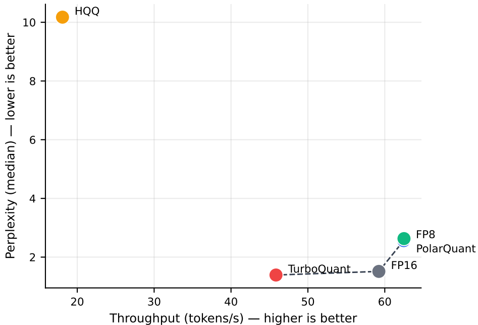
Quality vs decode speed @ 16,000 ctx
