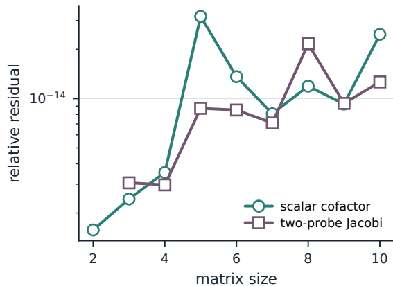
(c) Cofactor and Jacobi identities
