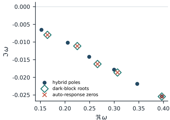
(a) Pole-zero structure in a multimode response
