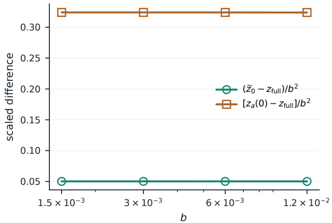
(b) Weak-field path at \bar{q}_0
