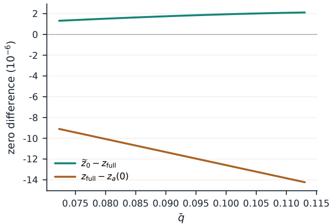
(a) Reduced-model momentum window
