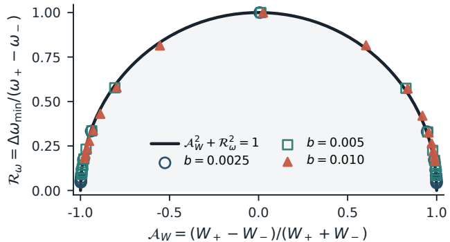
(b) Pole-weight circle law
