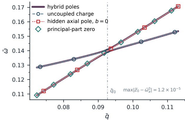
(a) Principal-part zero estimate
