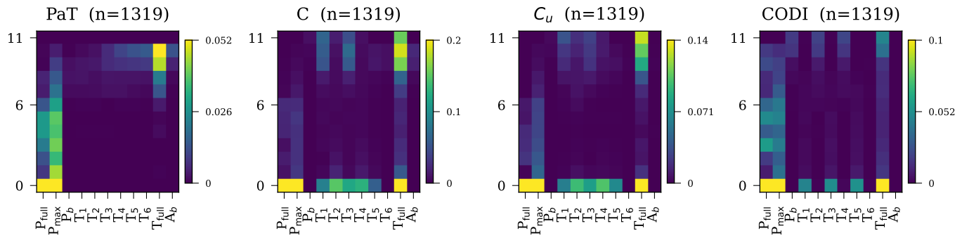
Arithmetic-Reasoning
