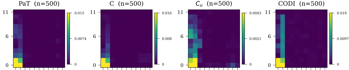
Graph-Hopping
