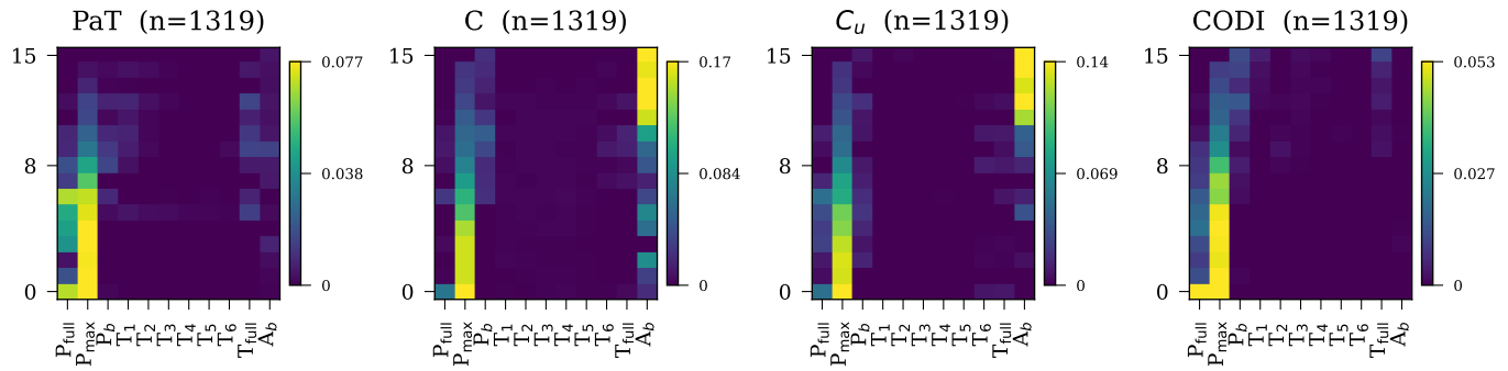
Arithmetic-Reasoning
