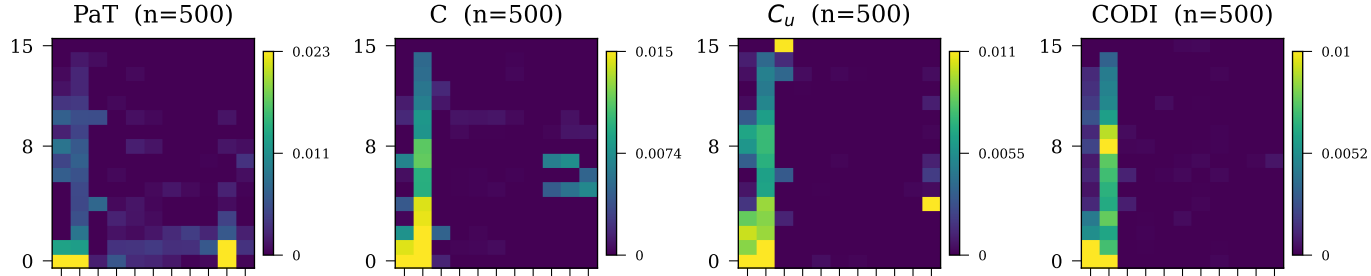
Graph-Hopping
