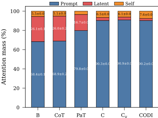
(a) Graph-Hopping
