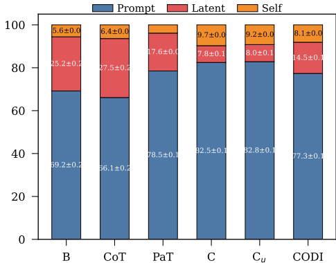
(b) Arithmetic-Reasoning
