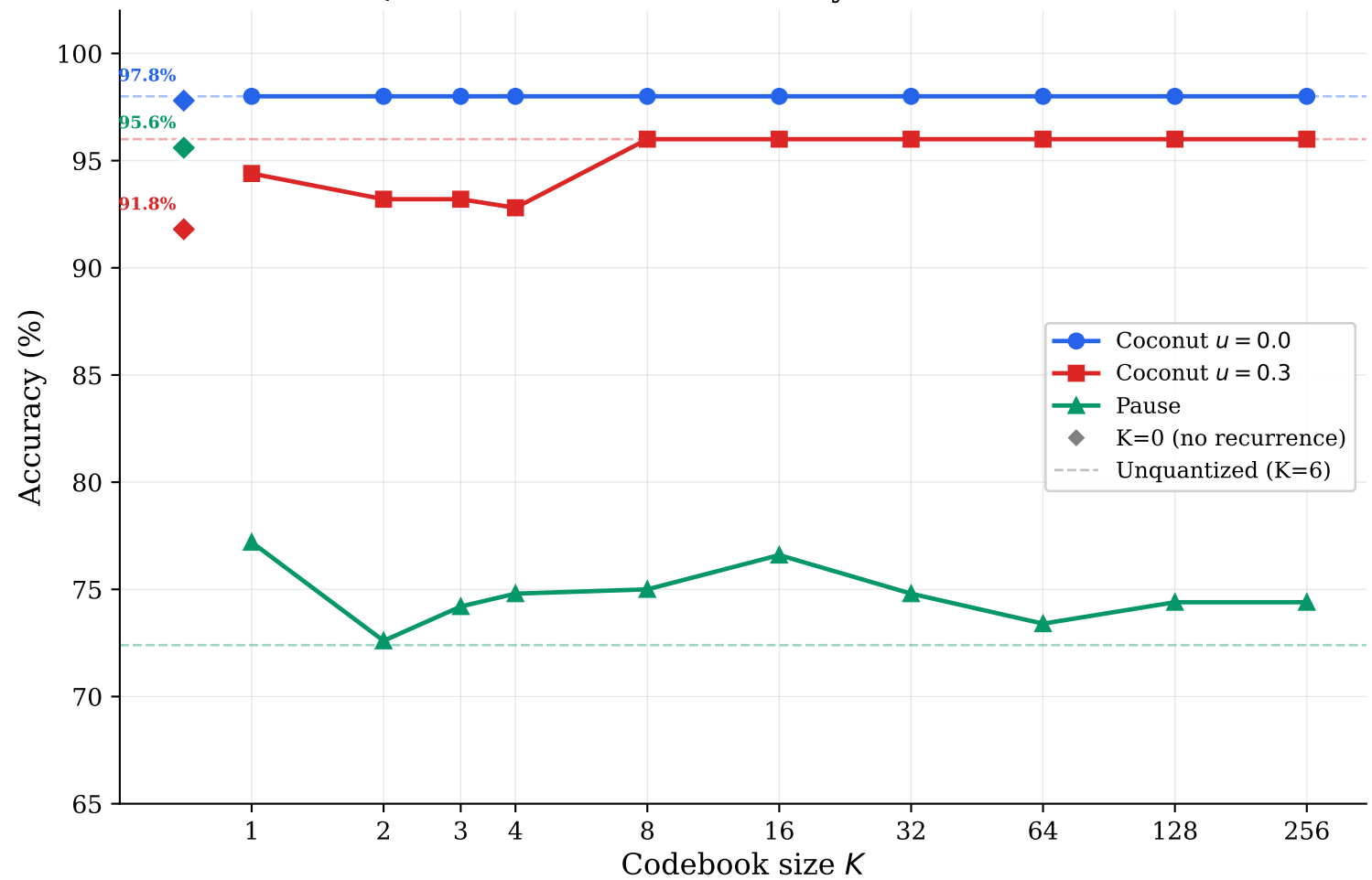
VQ-VAE Intervention: Accuracy vs Codebook Size
