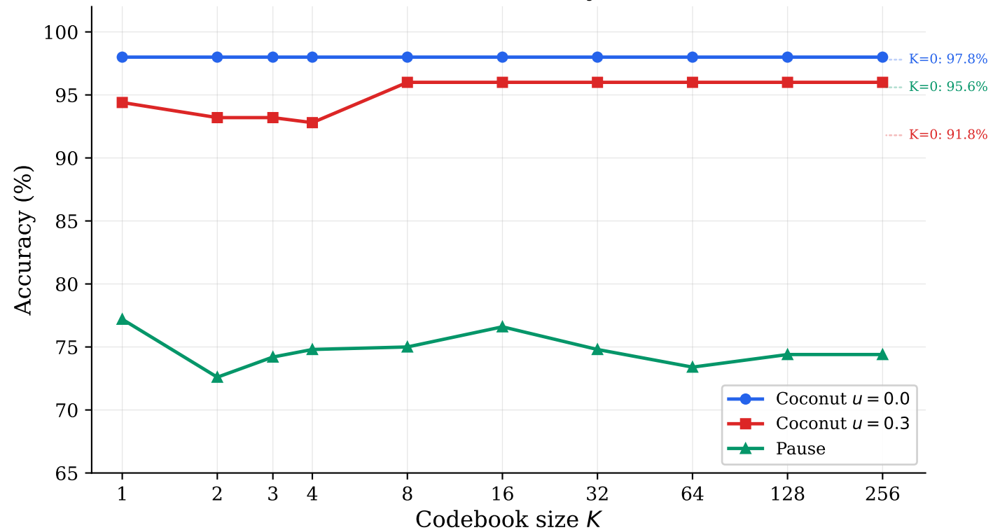
Quantized Recurrence: Accuracy vs Codebook Size
