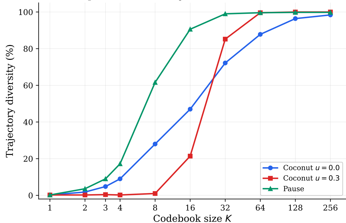
Unique Codebook Trajectories vs Codebook Size
