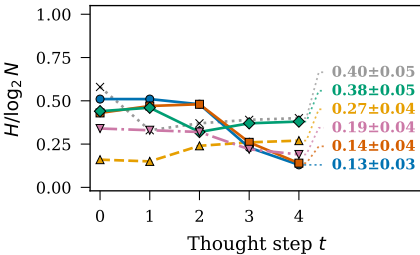
(a) Entropy
