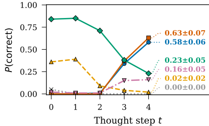
(b) P(\text{correct})
