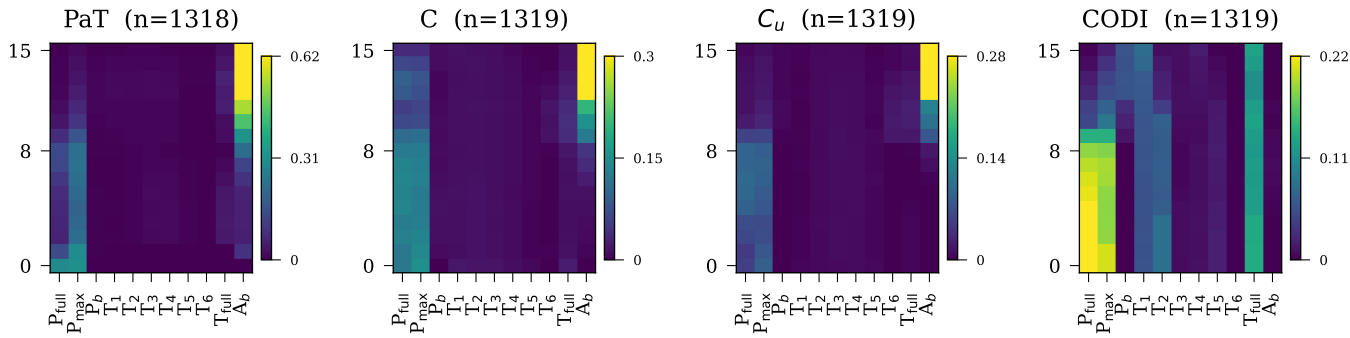
Arithmetic-Reasoning
