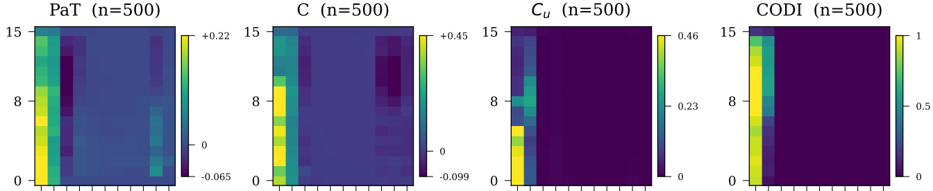
Graph-Hopping
