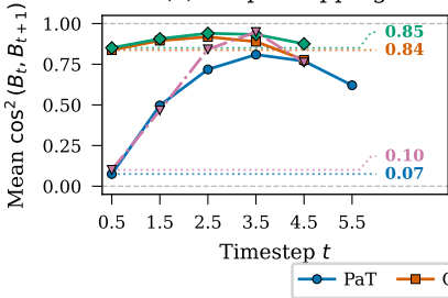
(a) Graph-Hopping
