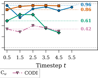
(b) Arithmetic-Reasoning
