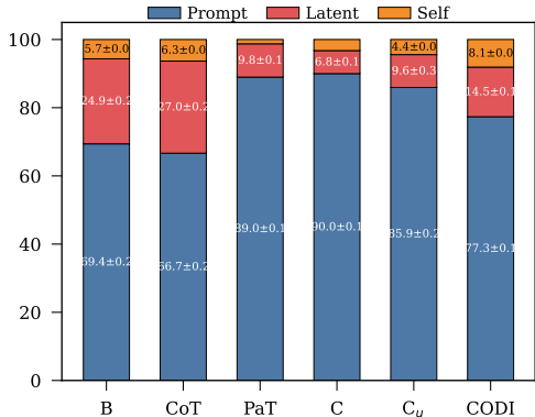
(b) Arithmetic-Reasoning
