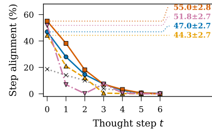
(f) Step Alignment
