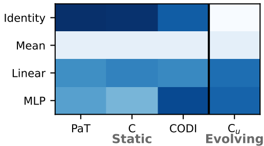
Graph-Hopping
