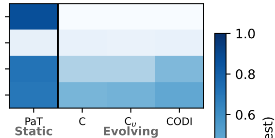
Arithmetic-Reasoning
