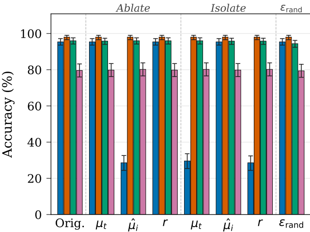
(a) Graph-Hopping
