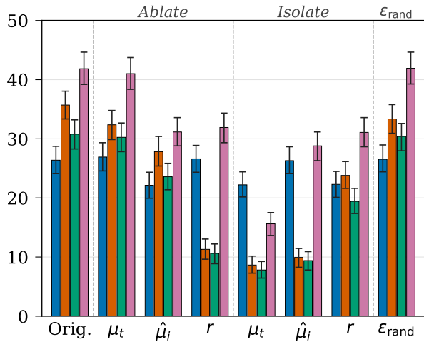
(b) Arithmetic-Reasoning
