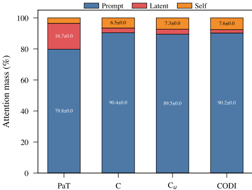
(a) Graph-Hopping
