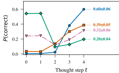
(b) P(\text{correct})
