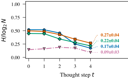
(a) Entropy
