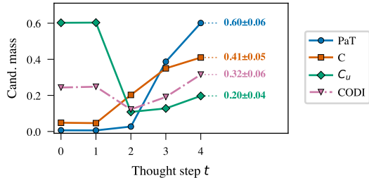
(c) Cand. Mass
