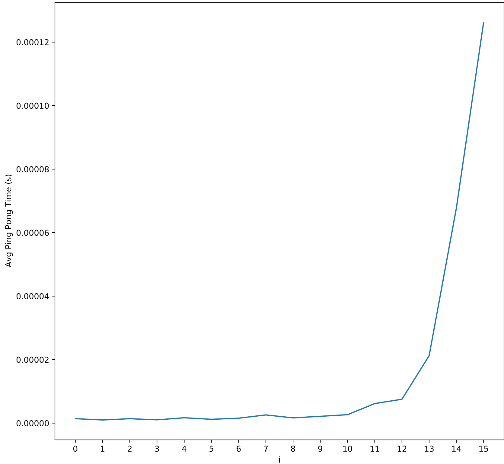
Problem 1 - Ping-Pong Time vs. Message Size ( 2^i )
