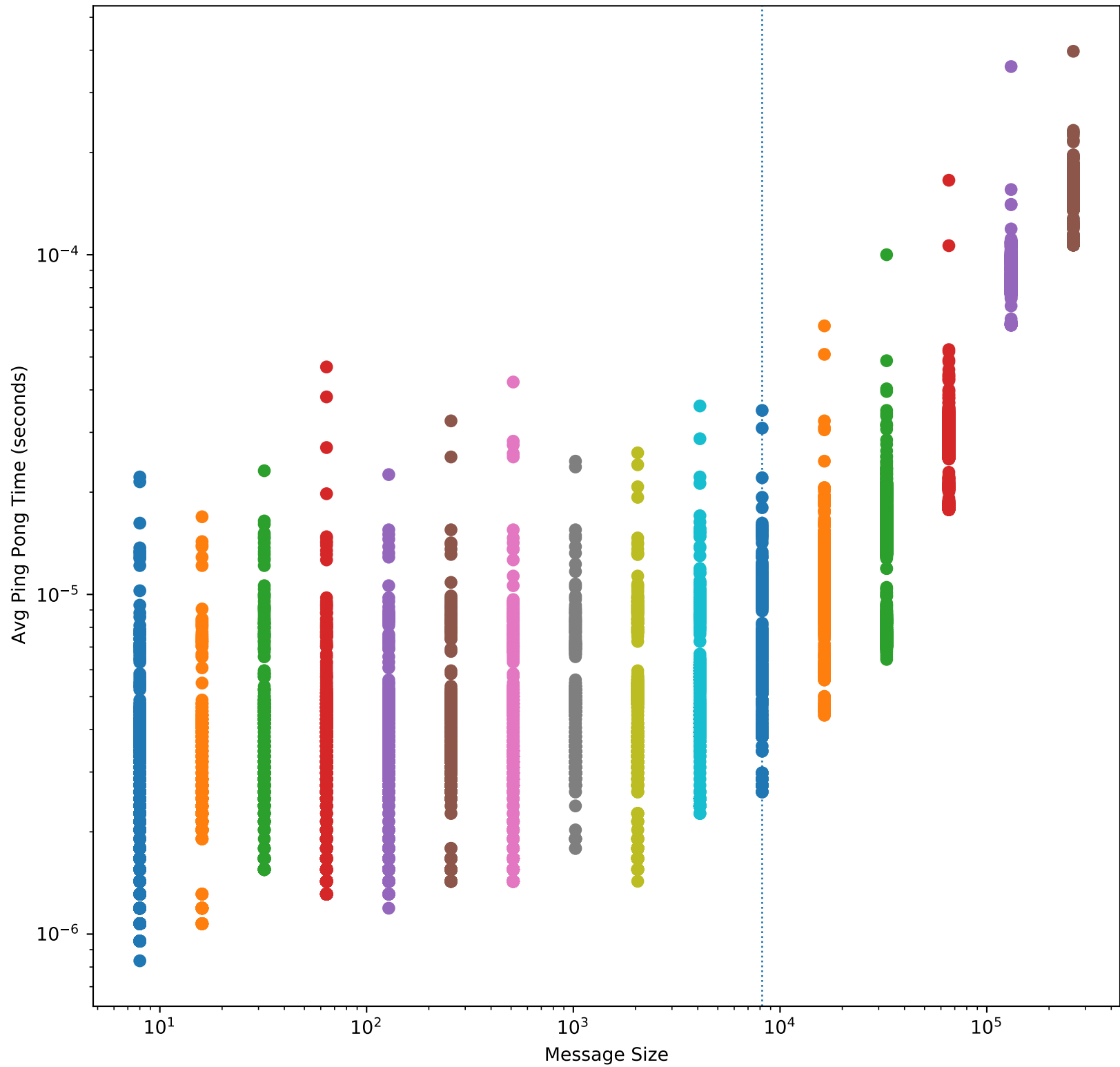
Problem 1 - Ping-Pong Time vs. Message Size
