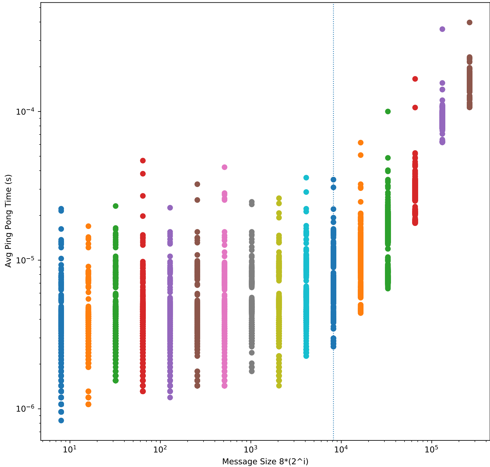
Problem 1 - Ping-Pong Time vs. Message Size 8\text{bytes} \cdot (2^i)
