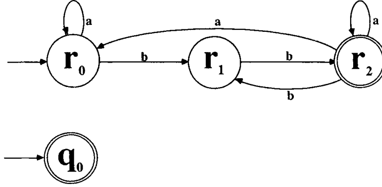
Figure 5.14: The resulting NFA for Example 5.16
