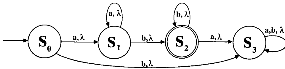
Figure 5.16: An automaton accepting Z(C) in Example 5.17
