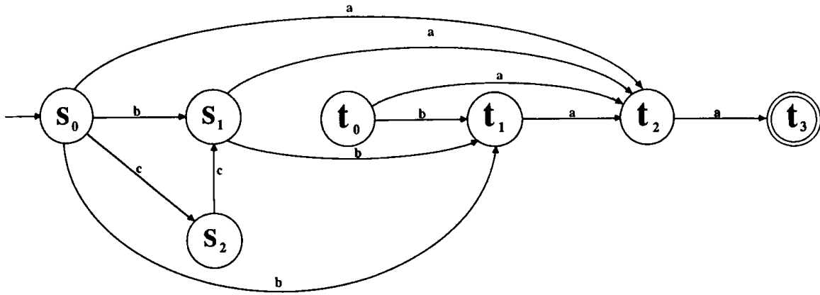
Figure 5.12: The concatenation of the NDFAs in Example 5.13
