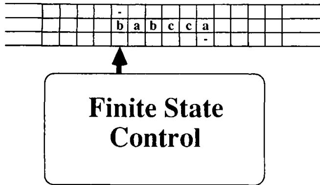
Figure 11.14a: A three-track Turing machine employing delimiters
