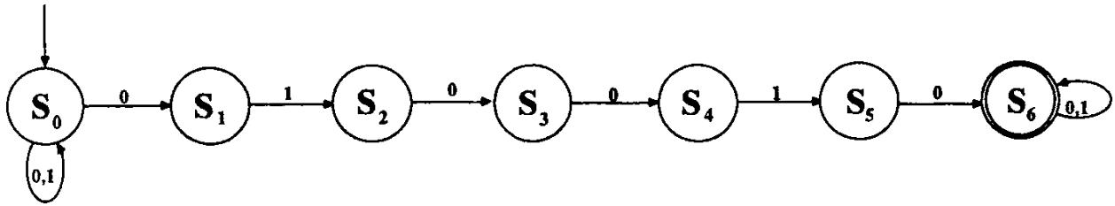
Figure 4.6: An NFA for pattern recognition
