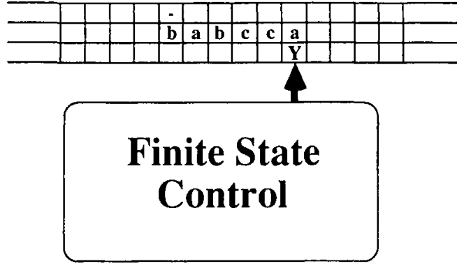
Figure 11.14b: An accepting configuration
