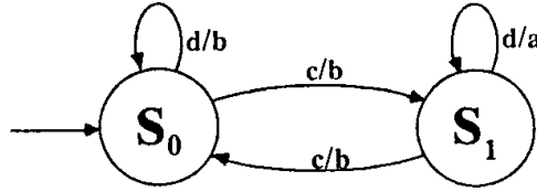
Figure 7.17: The state transition diagram for the Mealy machine in Example 7.17
