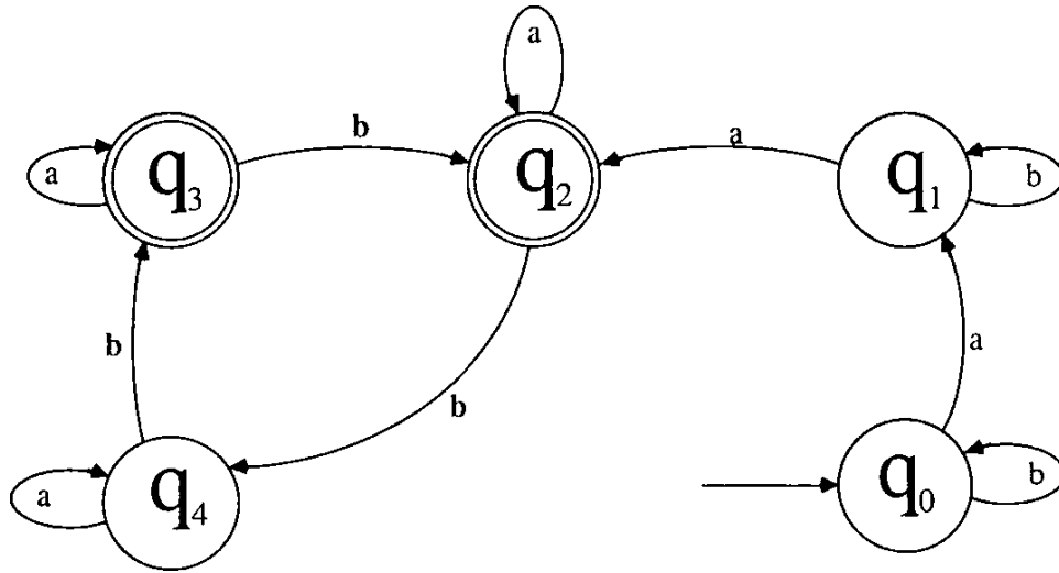
Figure 1.27: The DFA discussed in Exercise 1.1.23.
