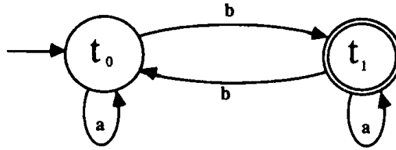
Figure 1.28: The DFA discussed in Exercise 1.1.29.
