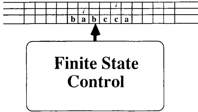
Figure 11.8: Emulating a two-headed Turing machine with a three-track tape
