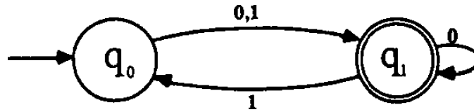
Figure 1.26: The automaton discussed in Exercise 1.1.3.
