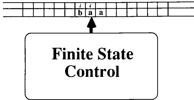
Figure 11.7: A Turing machine with a two-track tape
