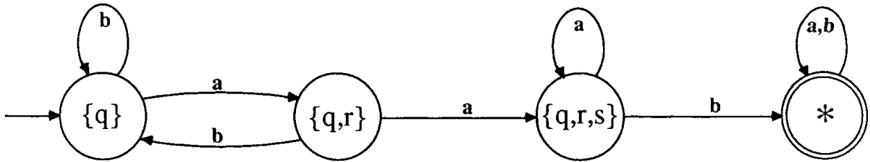
Figure 4.15: A reduced equivalent of the DFA given in Figure 4.14
