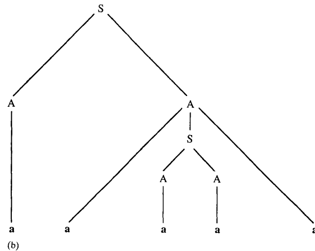
Figure 9.5: (a) A parse tree for aaaaa in Example 9.5 (b) An alternate parse tree for aaaaa
