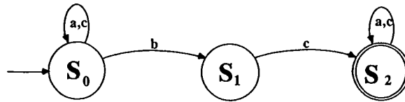
Figure 4.21: The NFA described in Example 4.16
