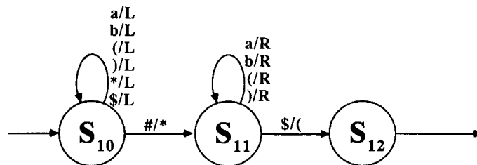
Figure 11.5b: Submachine S_1 in Example 11.4
