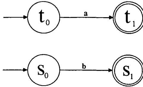
Figure 6.2: The NDFA discussed in Example 6.4
