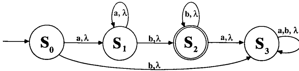
Figure 4.41: An automaton accepting Z(C) in Example 5.17
