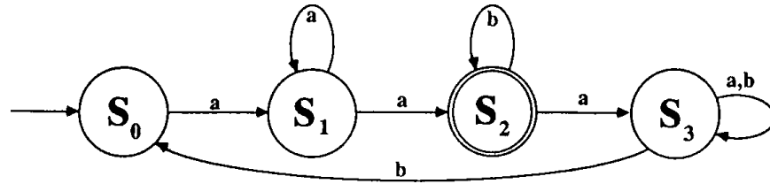
Figure 4.58: The automaton for Exercise 6.41
