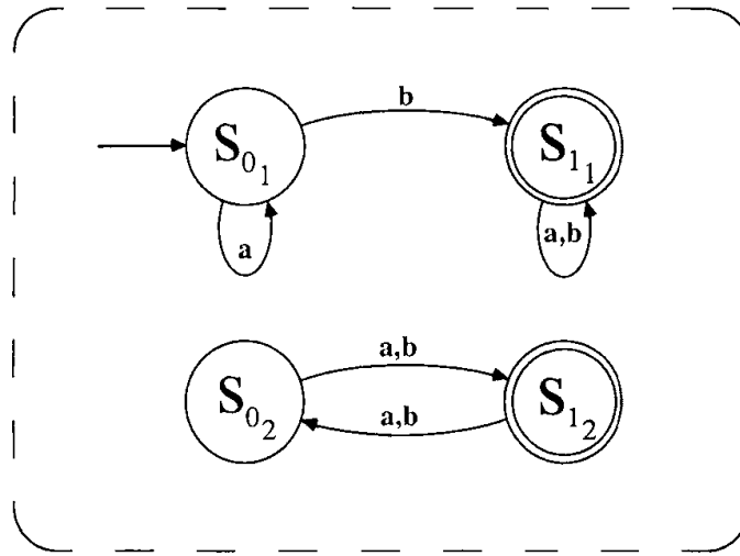
Figure 5.3: The composite machine discussed in Example 12.2
