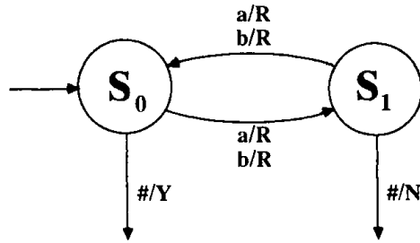
Figure 4.9: An alternate depiction of the Turing machine discussed in Example 11.1
