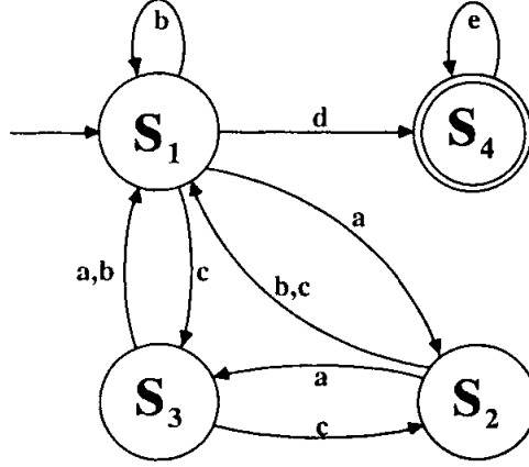
Figure 4.54: The DFA discussed in Example 6.12
