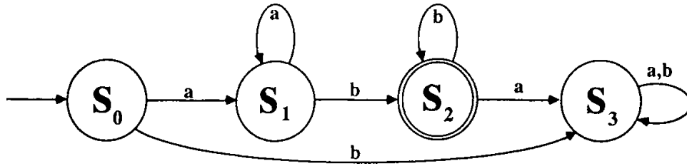
Figure 4.40: The automaton C discussed in Example 5.17
