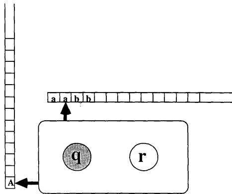
Figure 4.3b: Walkthrough of the pushdown automaton discussed in Example 10.1
