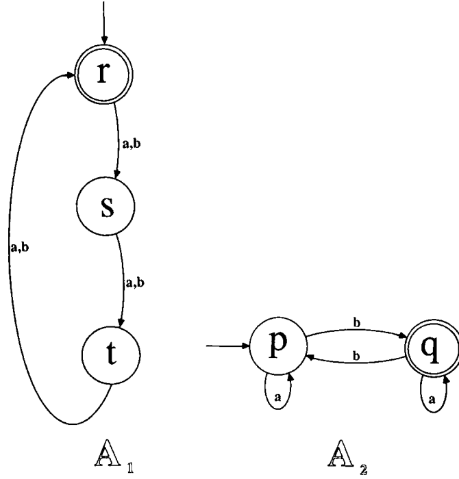
Figure 4.28: The automata discussed in Example 5.7
