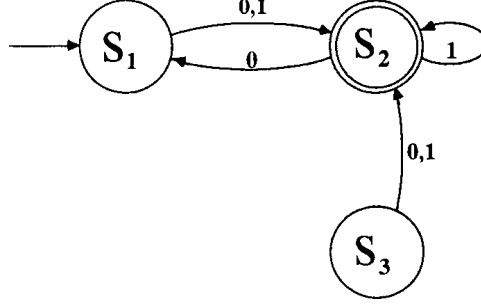
Figure 4.56: The DFA discussed in Exercise 6.19
