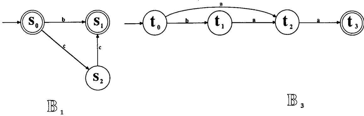
Figure 4.36: Candidates for concatenation in which the second machine does not accept \lambda (Example 5.13)
