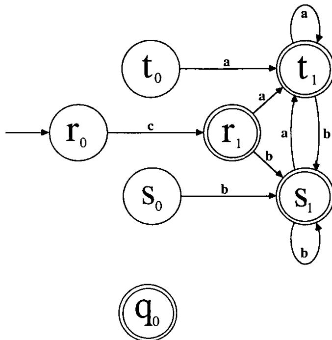
Figure 4.50: The NFA discussed in Example 6.6
