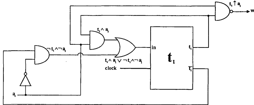
Figure 4.78: Circuit diagram for Example 7.17
