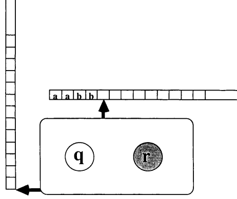
Figure 4.3e: Walkthrough of the pushdown automaton discussed in Example 10.1
