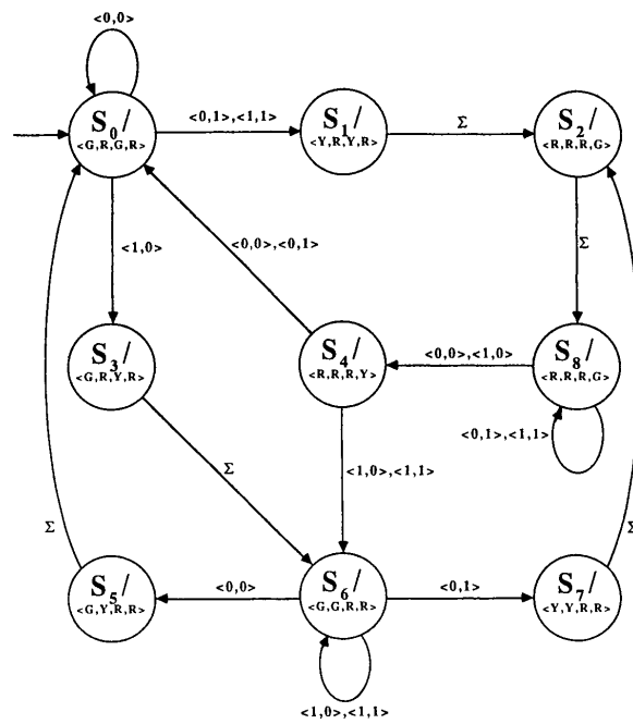
Figure 4.76: The modified controller discussed in Example 7.16
