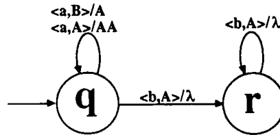
Figure 4.99: The PDA discussed in Example 10.1
