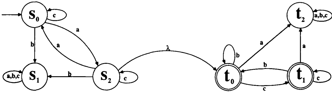
Figure 4.33: Concatenation of the machines in Example 5.10 via lambda-moves
