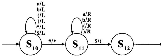
Figure 4.5b: Submachine S_1 in Example 11.4
