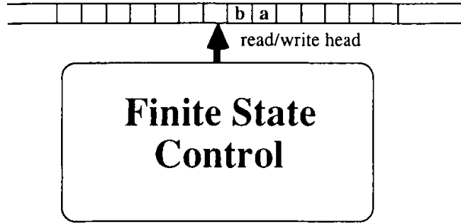
Figure 4.7: A model of a Turing machine.
