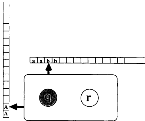
Figure 4.3c: Walkthrough of the pushdown automaton discussed in Example 10.1
