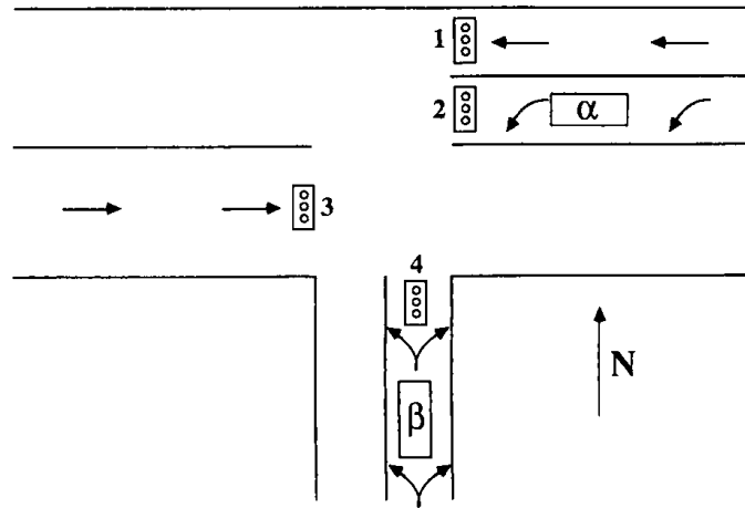
Figure 4.74: The intersection discussed in Example 7.16
