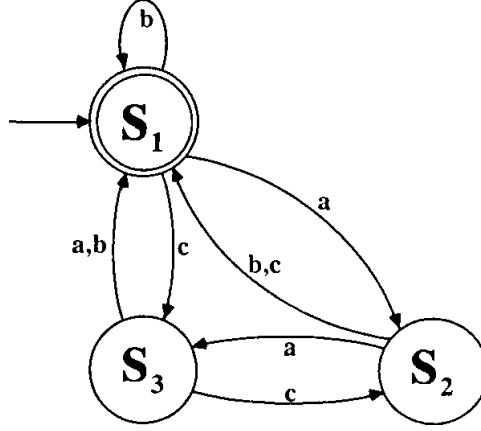
Figure 4.53: The DFA discussed in Example 6.11
