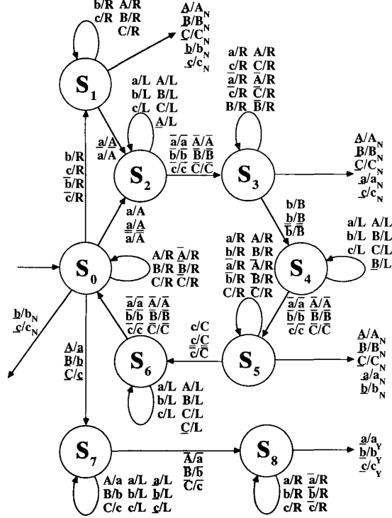
Figure 4.15: The Turing machine discussed in Example 11.13
