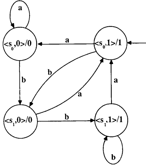
Figure 4.68: The state transition diagram for the Moore machine A in Example 7.12
