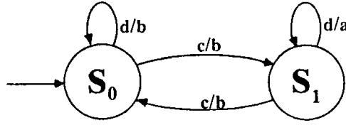
Figure 4.77: The state transition diagram for the Mealy machine in Example 7.17
