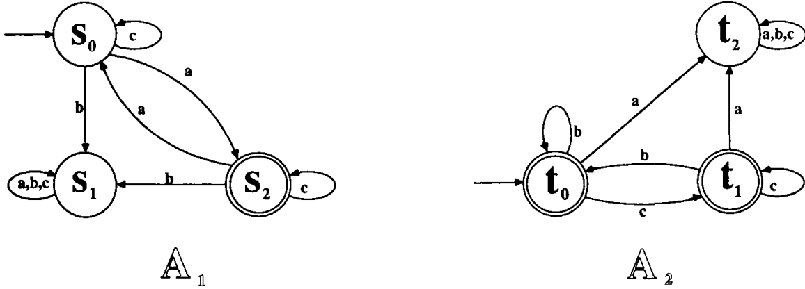
Figure 4.32: A pair of candidates for concatenation
