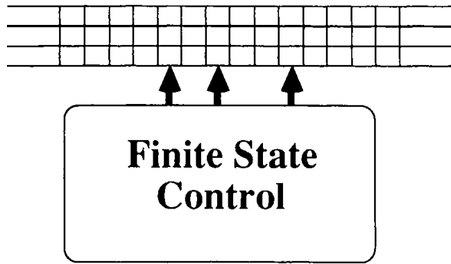
Figure 4.10: Emulating a three-tape Turing machine with a single three-track tape
