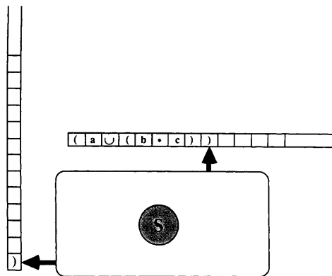
Figure 4.5f: Walkthrough of the pushdown automaton discussed in Example 10.7
