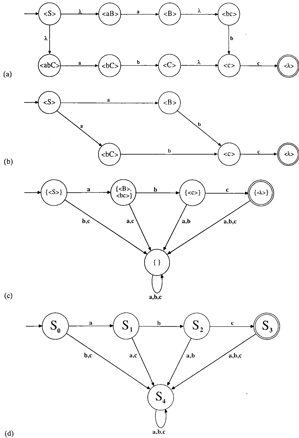
Figure 4.94: (a) The automaton discussed in Example 9.9 (b) The simplified automaton discussed in Example 9.9 (c) The deterministic automaton discussed in Example 9.9 (d) The final automaton discussed in Example 9.9
