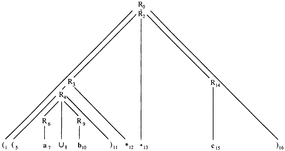
Figure 4.89: The preorder traversal of the parse tree
