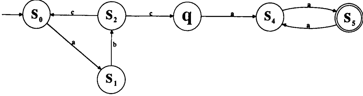
Figure 4.46: The automaton discussed in Example 5.25
