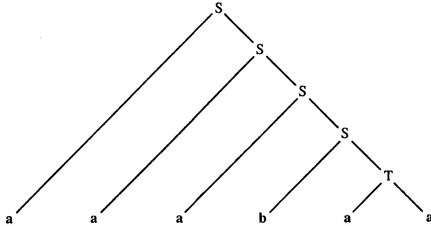
Figure 4.87: The parse tree discussed in Example 9.2
