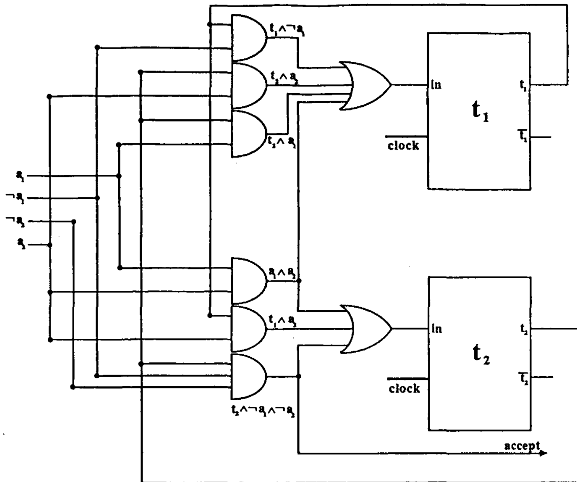
Figure 4.18: Circuitry for the automaton discussed in Example 4.13
