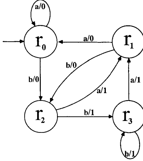
Figure 4.67: The state transition diagram for the Mealy machine M in Example 7.11
