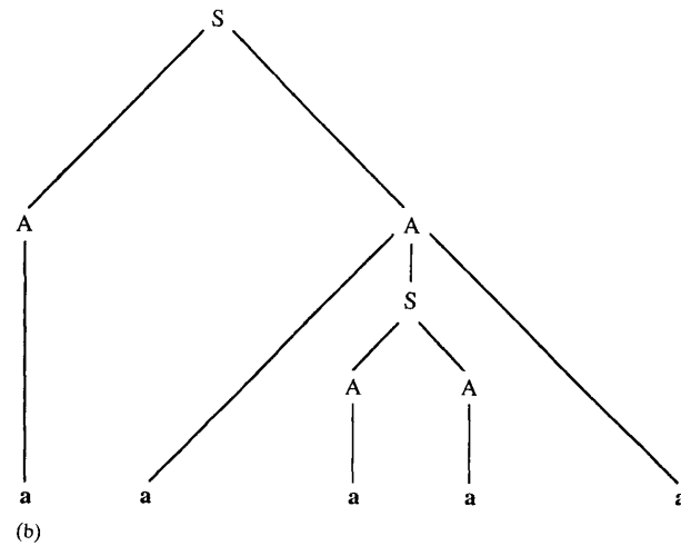
Figure 4.90: (a) A parse tree for aaaaa in Example 9.5 (b) An alternate parse tree for aaaaa
