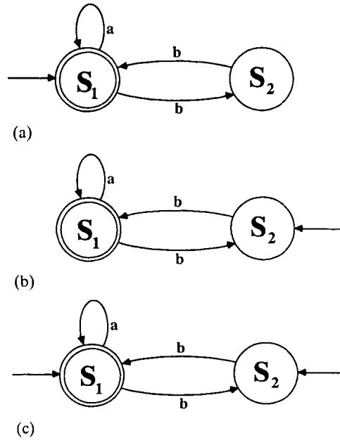
Figure 4.52: (a) The NFA B discussed in Example 6.10 (b) The NFA C discussed in Example 6.10 (c) The NFA D discussed in Example 6.10
