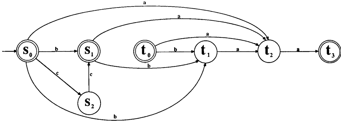
Figure 4.35: An NFA without lambda-moves which accepts the concatenation of the languages discussed in Example 5.8
