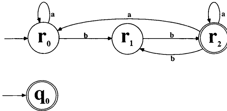
Figure 4.39: The resulting NDFA for Example 5.16
