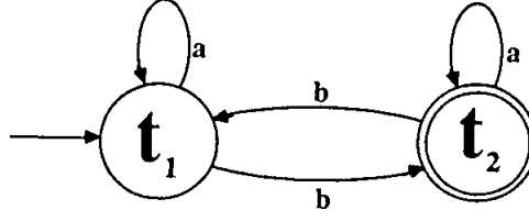
Figure 4.51: The DFA discussed in Example 6.9
