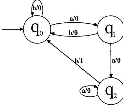
Figure 4.65: The state transition diagram for the Mealy machine D in Example 7.8
