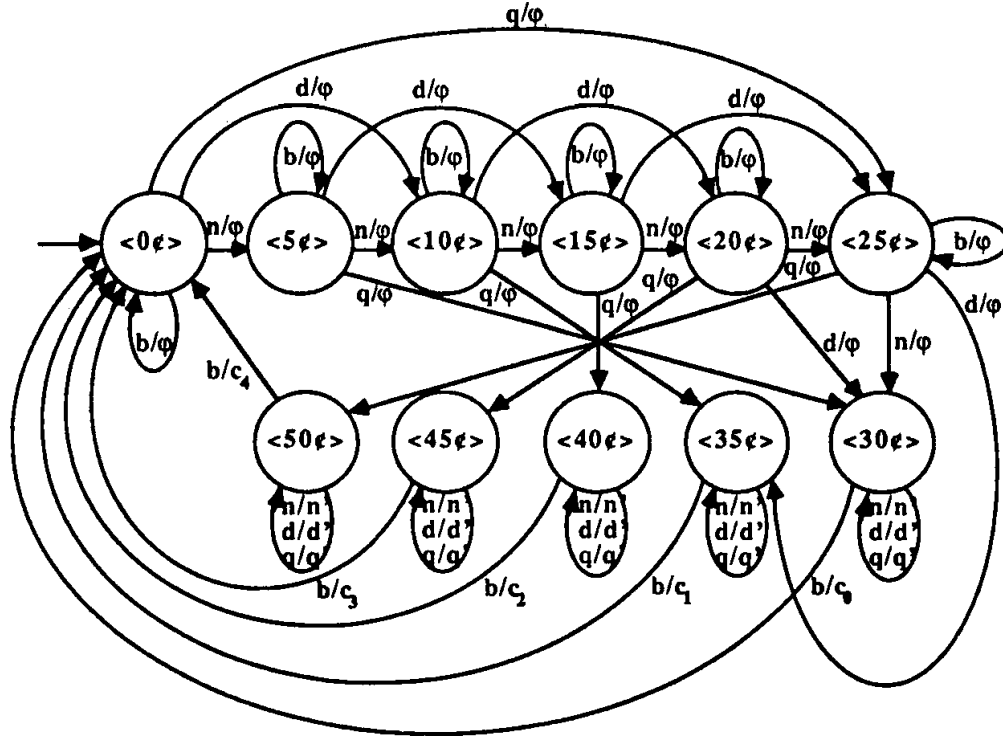
Figure 4.62: A finite-state transducer model of the vending machine discussed in Example 7.1
