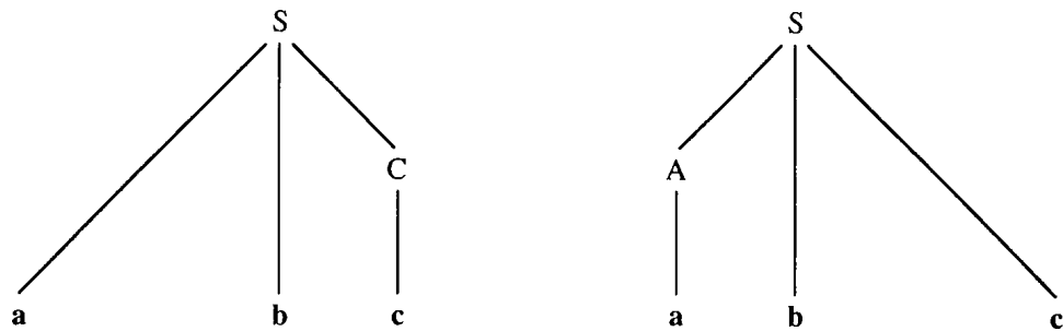
Figure 4.93: The parse trees discussed in Example 9.8
