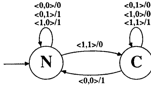
Figure 4.73: The state transition diagram for a binary adder modeled as a Mealy machine, as discussed in Example 7.15
