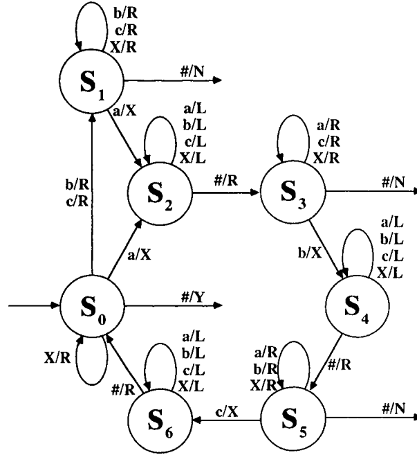
Figure 4.10: The Turing machine M discussed in Example 11.2
