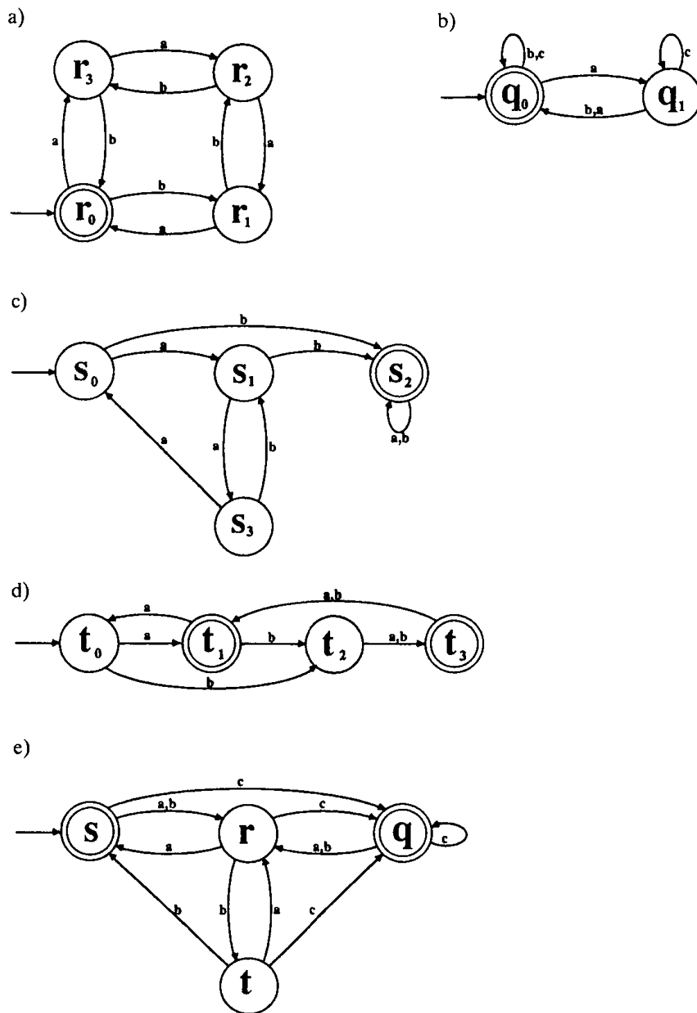
Figure 4.84: Automata for Exercise 8.31
