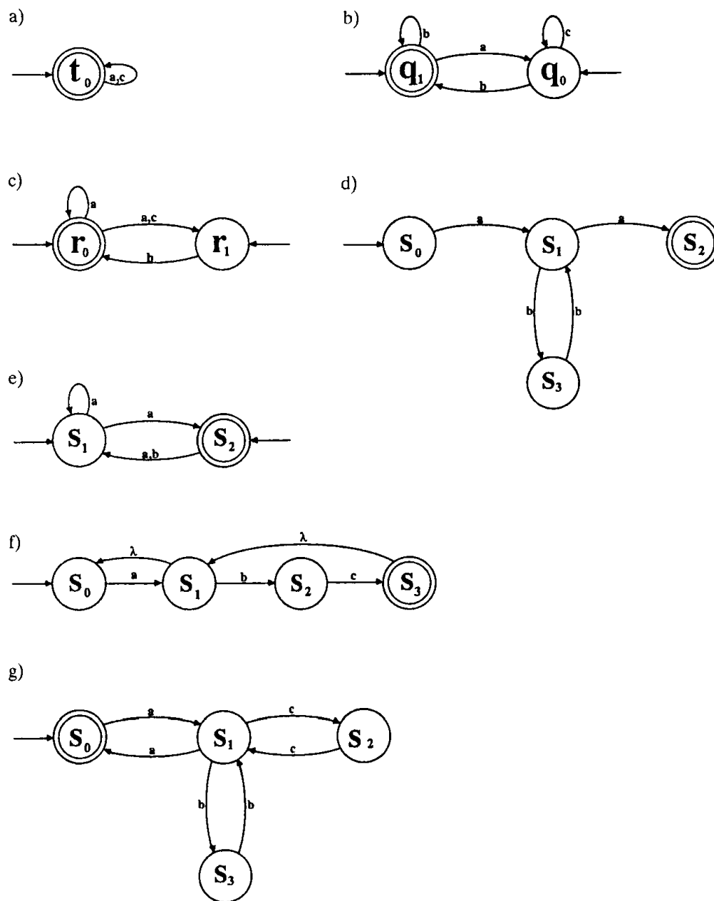
Figure 4.85: Automata for Exercise 8.32
