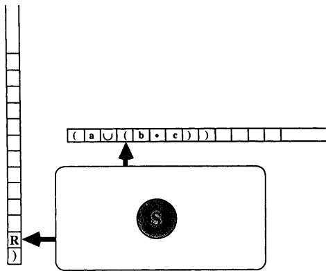
Figure 4.5d: Walkthrough of the pushdown automaton discussed in Example 10.7
