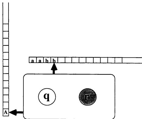
Figure 4.3d: Walkthrough of the pushdown automaton discussed in Example 10.1
