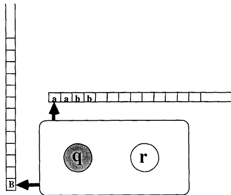
Figure 4.3a: Walkthrough of the pushdown automaton discussed in Example 10.1
