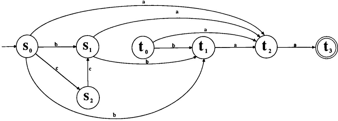
Figure 4.37: The concatenation of the NDFAs in Example 5.13
