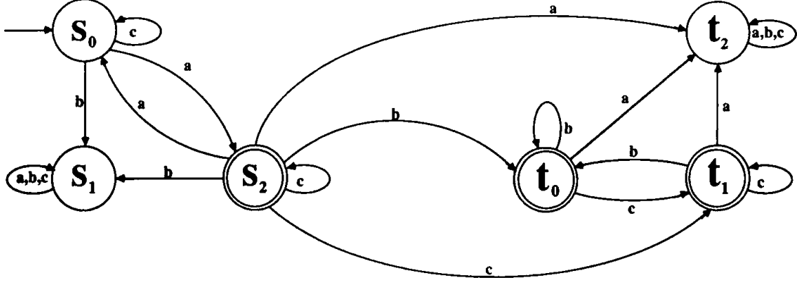
Figure 4.34: Concatenation of the machines in Example 5.10 without lambda-moves (Example 5.11)
