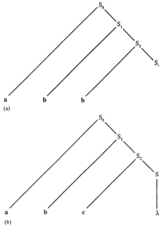
Figure 4.95: (a) The partial parse tree for the string abb (b) The parse tree for the string abc
