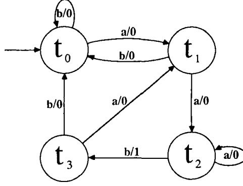
Figure 4.64: The state transition diagram for the Mealy machine C in Example 7.6
