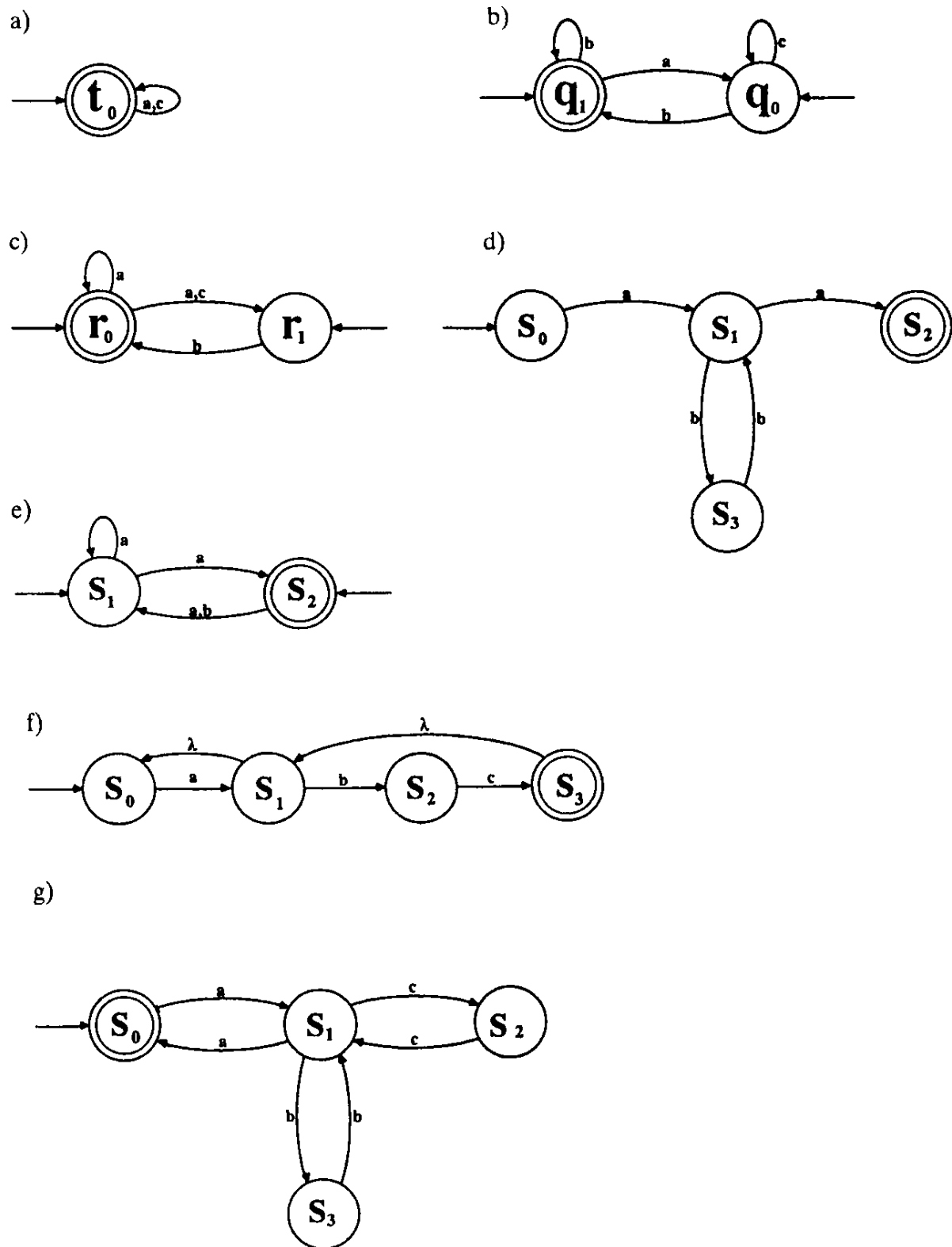
Figure 4.60: The automata for Exercise 6.50
