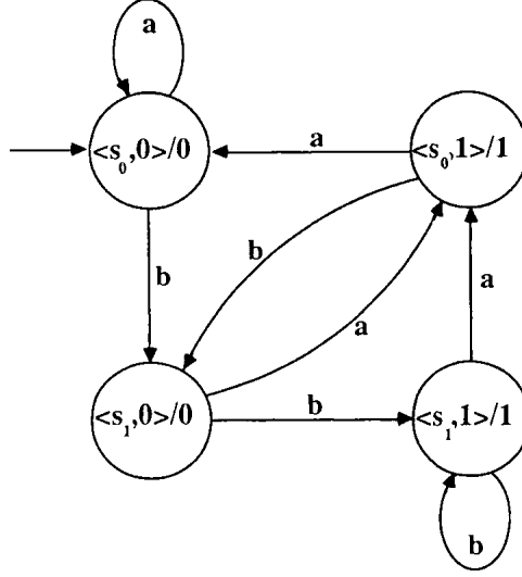
Figure 4.69: The state transition diagram for the Moore machine A' in Example 7.12
