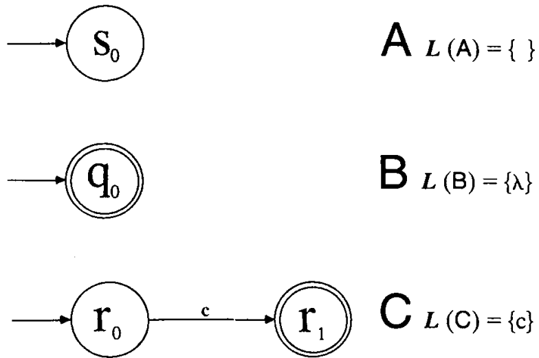
Figure 4.47: NDFAs which recognize regular expressions with zero operators
