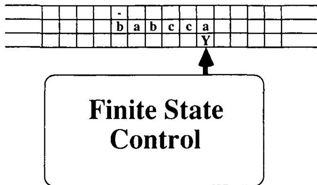
Figure 4.14b: An accepting configuration
