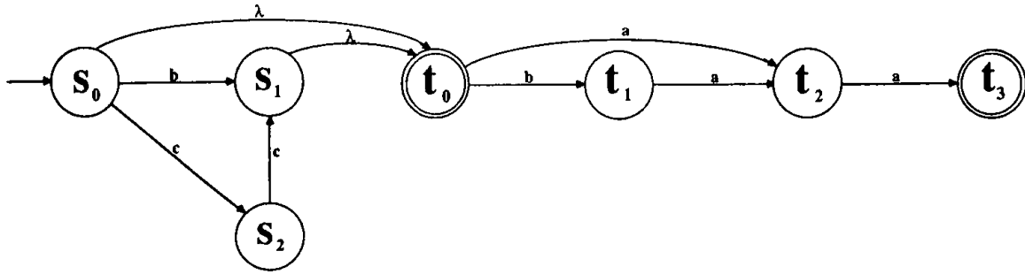
Figure 4.31: An NFA which accepts the concatenation of the machines discussed in Example 5.9
