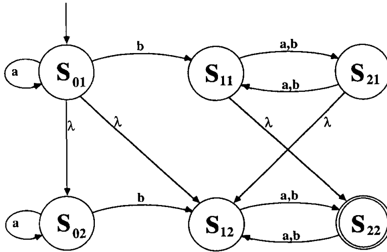
Figure 4.43: The modified machine in Example 5.18
