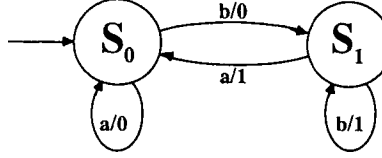
Figure 4.63: The state transition diagram for the transducer discussed in Example 7.2
