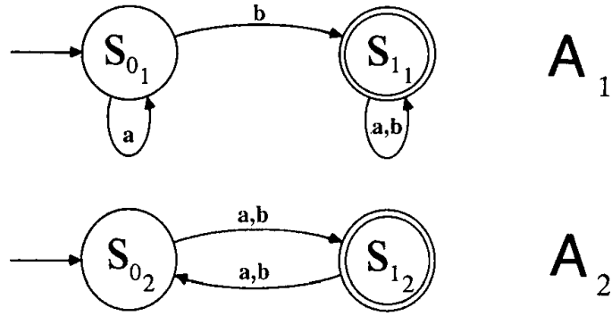
Figure 5.2: The automata discussed in Example 12.2
