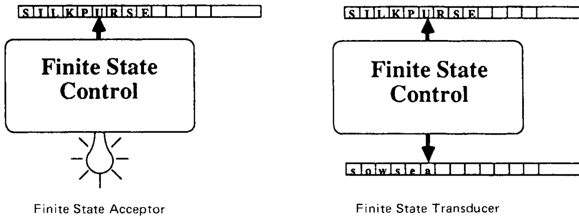
Figure 4.61: The difference between an acceptor and a transducer
