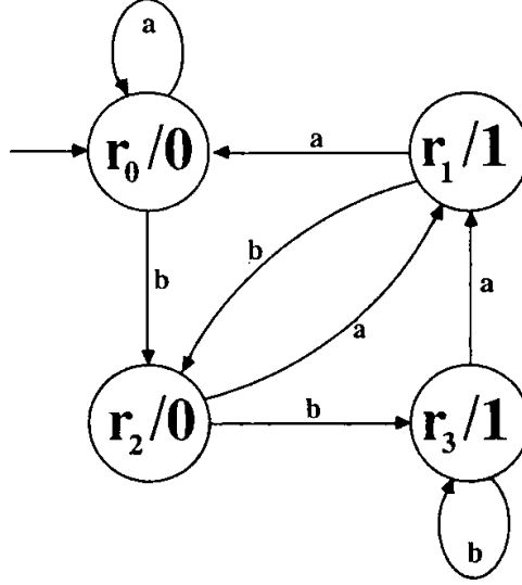
Figure 4.66: The state transition diagram for the transducer discussed in Example 7.10
