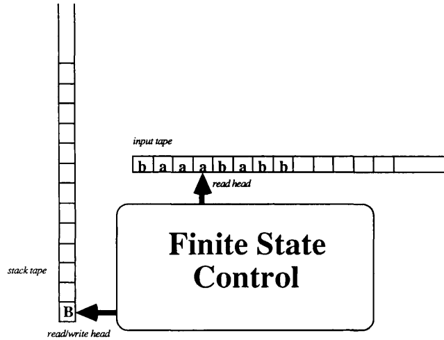
Figure 4.98: A model of a pushdown automaton
