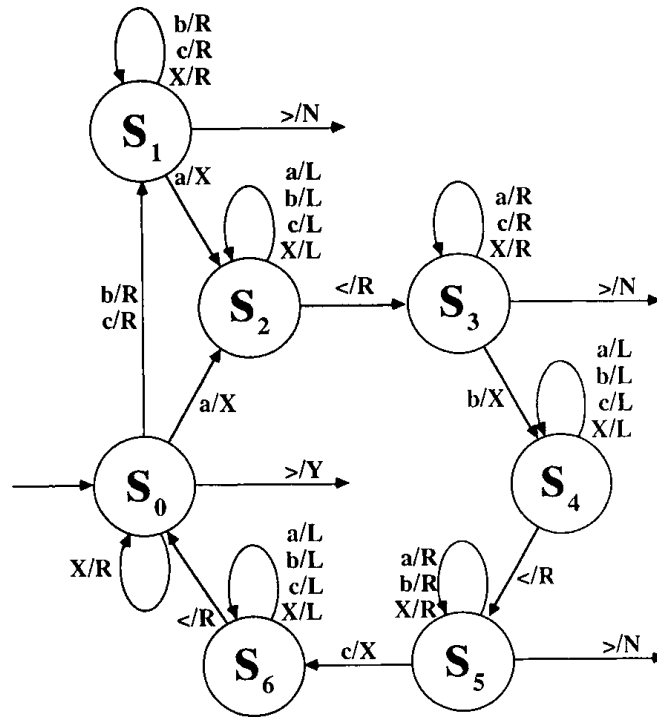
Figure 4.11: The Turing machine discussed in Example 11.10
