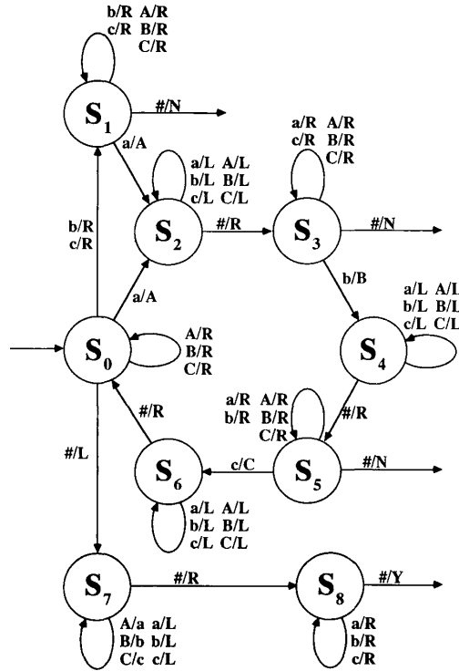
Figure 4.13: The state transition diagram discussed in Example 11.11
