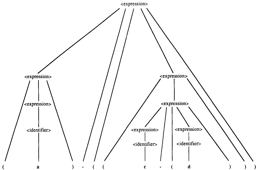
Figure 4.92: The parse tree discussed in Example 9.7
