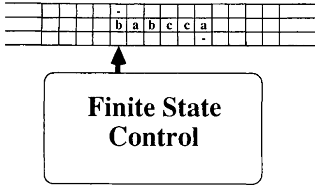
Figure 4.14a: A three-track Turing machine employing delimiters
