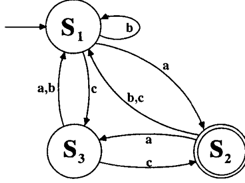
Figure 4.55: The DFA discussed in Example 6.13
