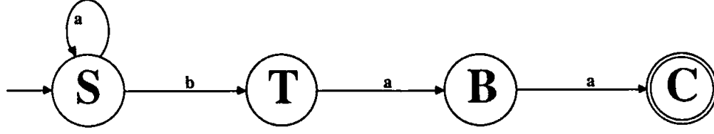
Figure 4.83: An automaton corresponding to a grammar in normal form
