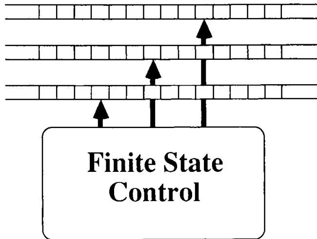
Figure 4.9: A three-tape Turing machine
