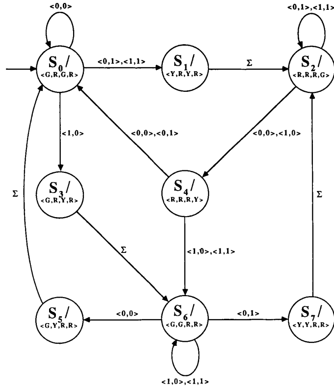
Figure 4.75: The state transition diagram for a stoplight modeled as a Moore machine, as discussed in Example 7.16
