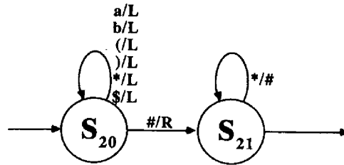
Figure 4.5c: Submachine S_2 in Example 11.4
