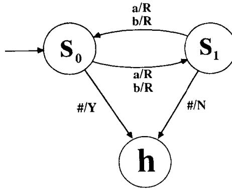
Figure 4.8: The state transition diagram of the Turing machine discussed in Example 11.1
