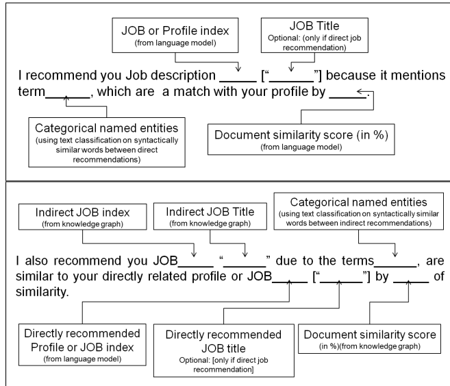
Fig. 4. Sentence template for the direct (above) and extended (below) recommended job explanation.
