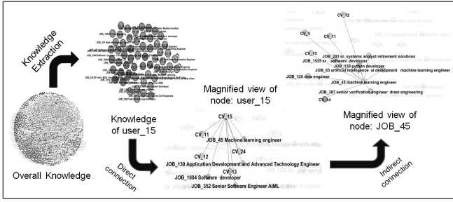
Fig. 3. The diagram shows the overview of the knowledge graph recommendations: Here, the knowledge of user profile 15 is extracted, in which user profile 15 is directly connected to four profiles and four job descriptions. These directly connected profiles and jobs are again connected directly to other jobs and profile (i.e. job 45), which are indirectly recommended for the user profile 15.
