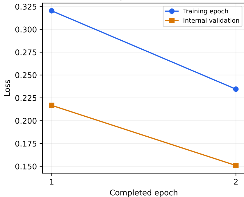
DPO preference loss
