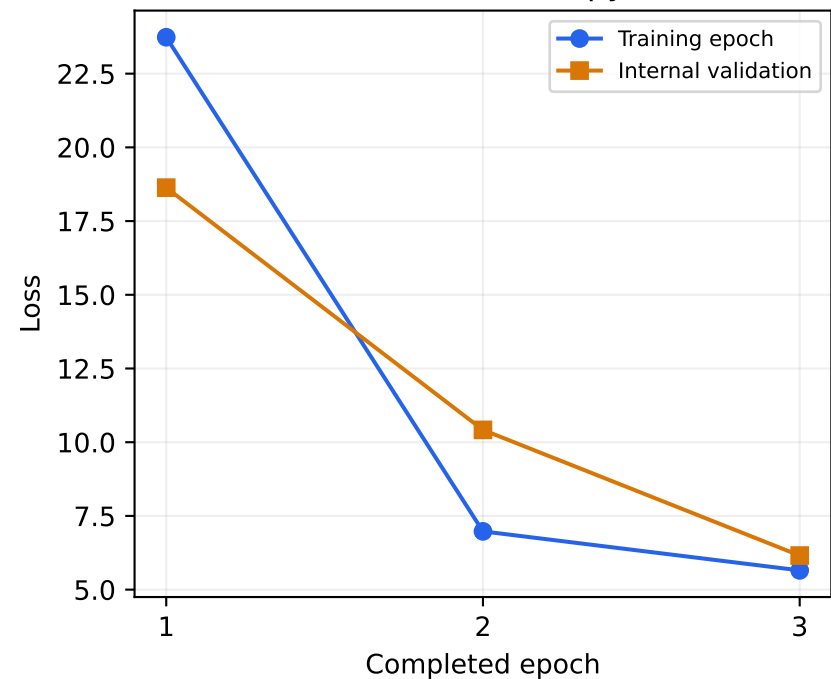
SFT cross-entropy
