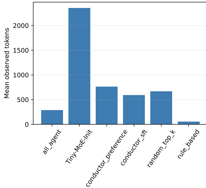
Heldout development tasks: identical task set and aggregate budgets
