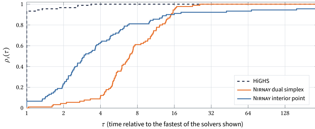
Figure 12: Dolan–Moré performance profile on the 90 Netlib problems. Times come from netlib_simplex_v4.csv and netlib_ipm_v2.csv . The two sweeps ran under different machine load (HiGHS itself was 0.7 times slower, in geometric mean, in the first than in the second), so each engine’s time is rescaled by the ratio of the common HiGHS time (the geometric mean of its two measurements) to HiGHS’s time in that engine’s sweep. HiGHS is fastest on a fraction 0.93 of the problems. The dual simplex is within a factor of 10 of the fastest on a fraction 0.67 and within 26 on all of them. The interior-point method’s curve stays below 1 because of its failures.
