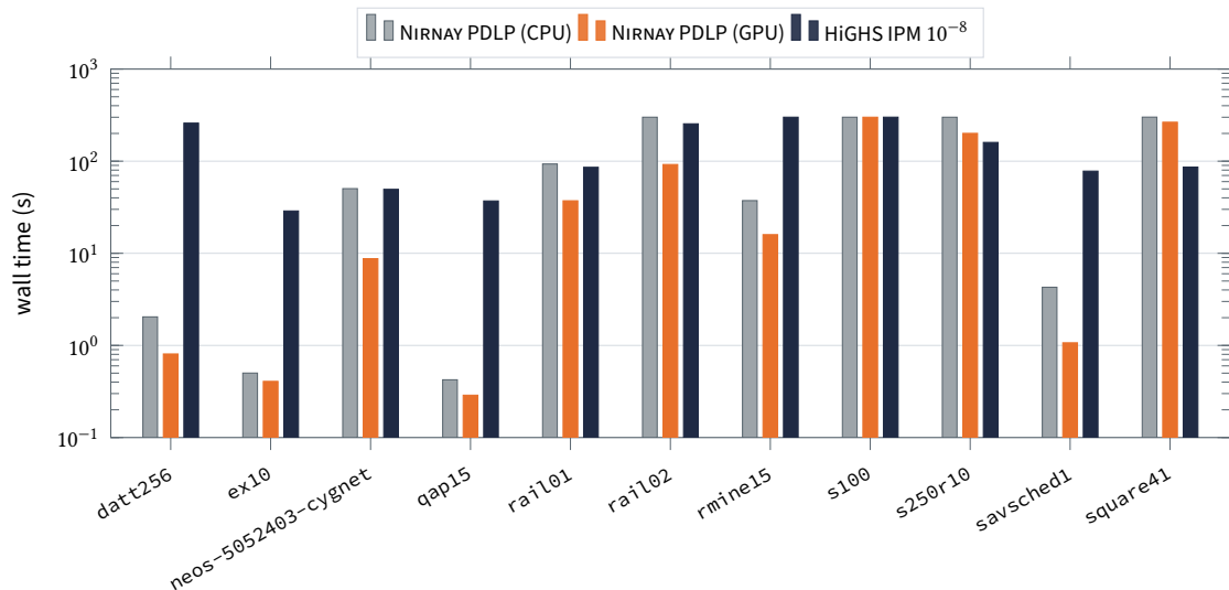
Figure 8: Wall time on the large LPs (log scale), from results/large_pdlp_gpu.csv . The PDLP runs stop at relative tolerance 10^{-4} ; the HiGHS reference solves to 10^{-8} .
