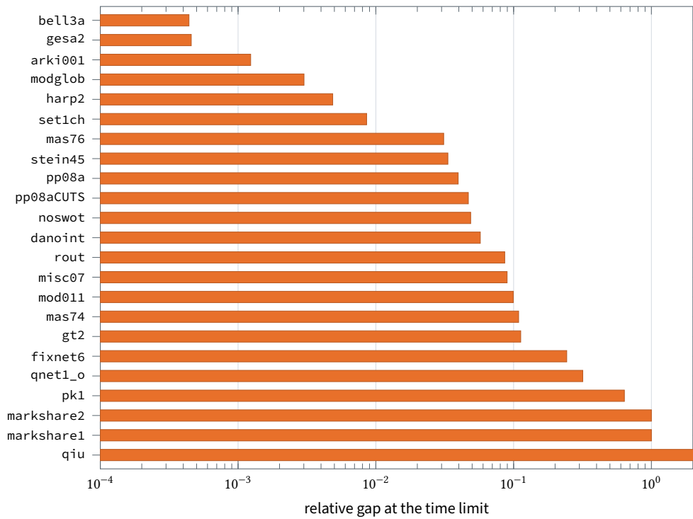
Figure 15: MIPLIB 3 instances that reached the 60 s limit with an incumbent: relative gap |f - \underline{z}| / \max(1, |f|) at the limit (log scale). The target is 10^{-4} .
