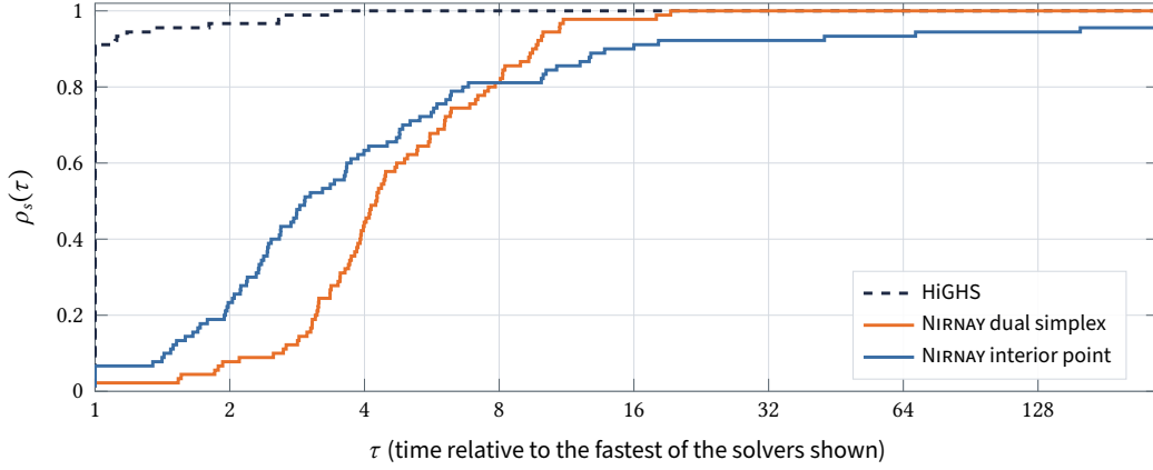
Figure 12: Dolan–Moré performance profile on the 90 Netlib problems. Times come from netlib_simplex_v5.csv and netlib_ipm_v2.csv . The two sweeps ran under different machine load (HiGHS itself was 0.7 times slower, in geometric mean, in the first than in the second), so each engine’s time is rescaled by the ratio of the common HiGHS time (the geometric mean of its two measurements) to HiGHS’s time in that engine’s sweep. HiGHS is fastest on a fraction 0.91 of the problems. The dual simplex is within a factor of 10 of the fastest on a fraction 0.93 and within 19 on all of them. The interior-point method’s curve stays below 1 because of its failures.
