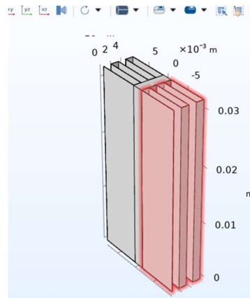
Figure 11: Reduced geometry of one tube and two fin channels (Iteration 6).
