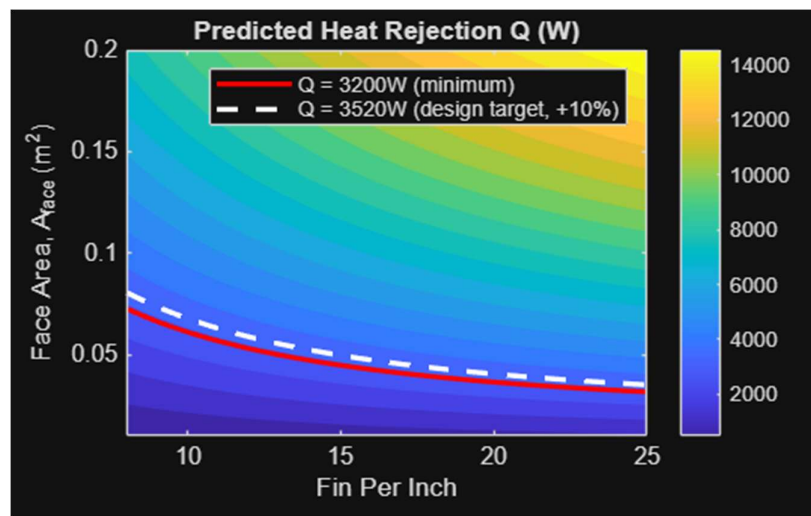
Figure 3: Predicted heat rejection Q(W) over the f_{\text{pi}} / A_{\text{face}} design grid, with the Q_{\text{target}} and +10% margin contours overlaid.
