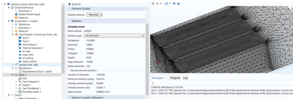
Figure 9: Mesh statistics after the swept mesh was added in Iteration 2.
