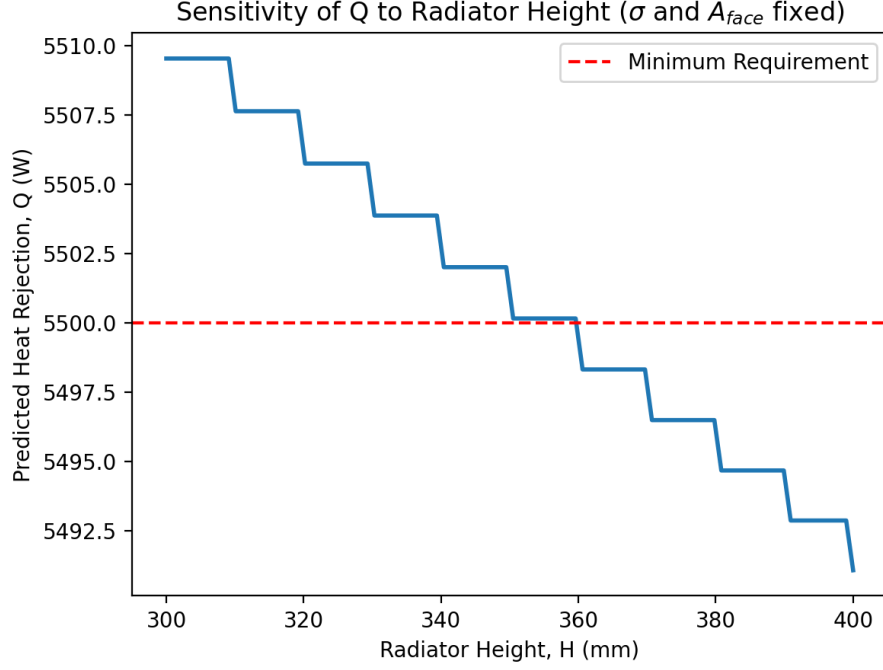
Figure 3: Sensitivity of predicted heat rejection to core height H , with fin density and face area held fixed at the chosen design point.
