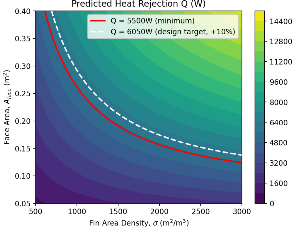
Figure 1: Predicted heat rejection Q across the swept fin area density ( \sigma ) and face area ( A_{\text{face}} ) design space. The red line marks the 5500 W minimum requirement; the white dashed line marks the 6050 W design target with 10% margin.
